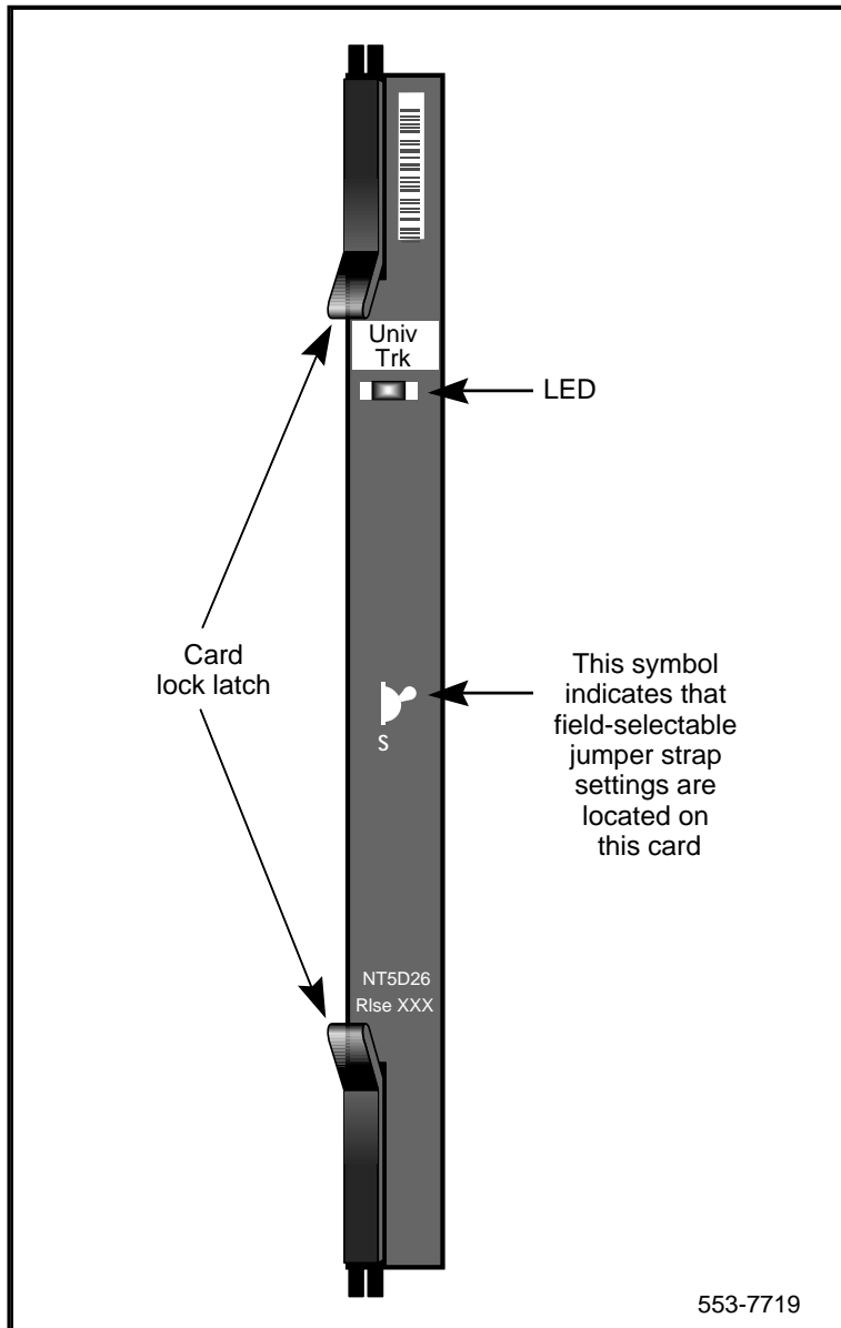
Figure 1 NT5D26 EXUTAP-1 and EXUTAP-2 Universal Trunk card—faceplate
