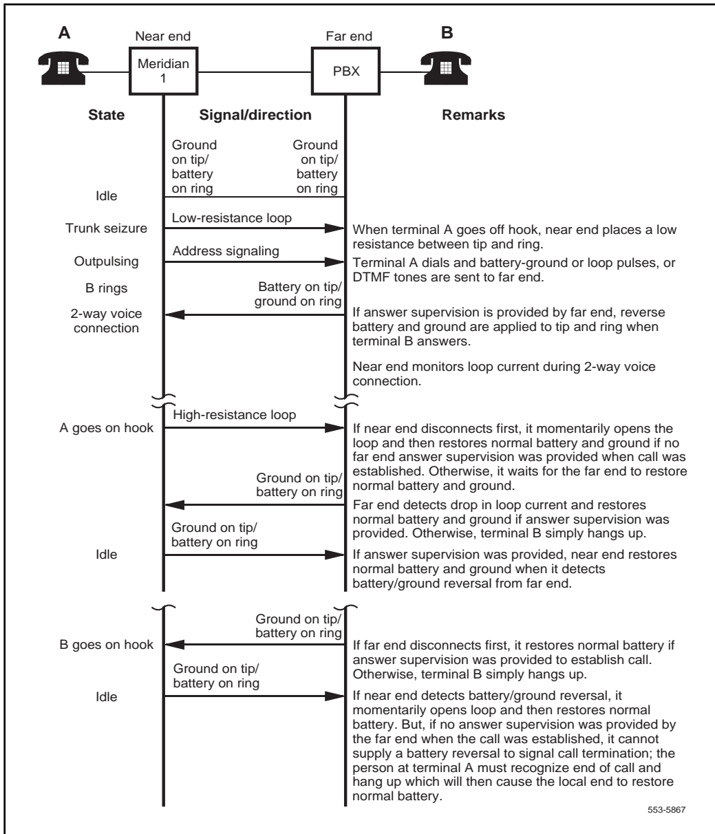
Figure 45 Two-way, Loop DR, TIE trunk call connection sequence – outgoing call to far-end PBX
