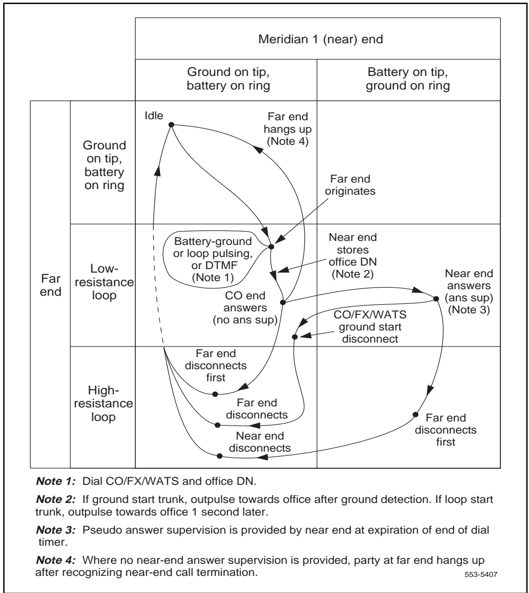
Figure 19 Two-way, Loop DR, TIE trunk call states—incoming call through senderized, tandem PBX from a CO/FX/WATS trunk
