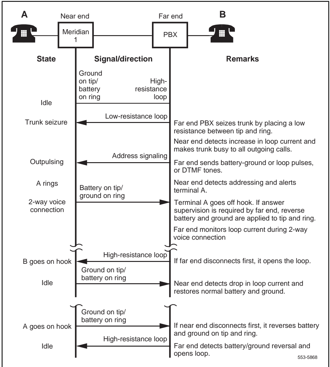
Figure 49 Two-way, loop OAID, TIE trunk call connection sequence – incoming call from far-end PBX
