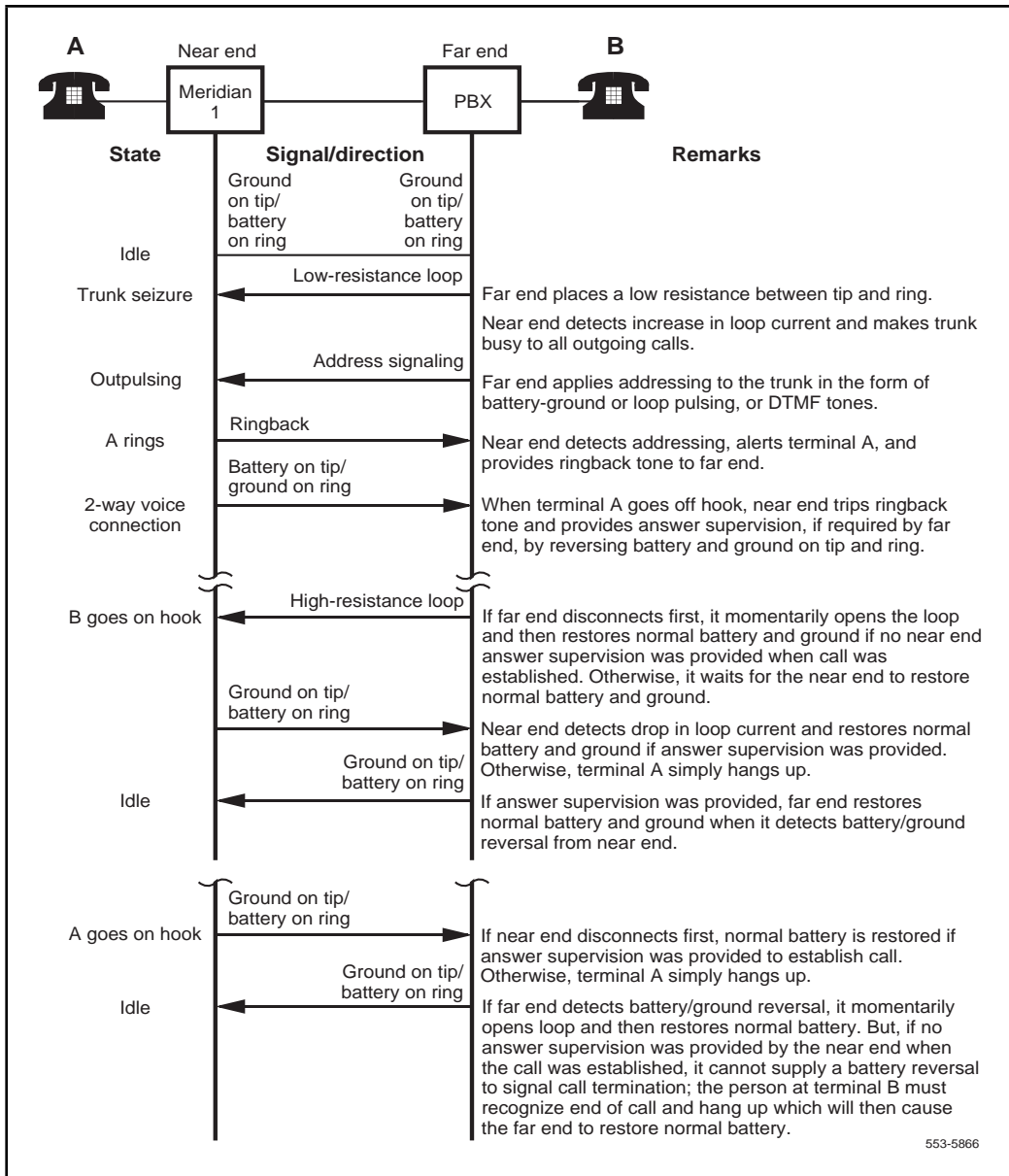
Figure 43 Two-way, Loop DR, TIE trunk call connection sequence – incoming call from far-end PBX
