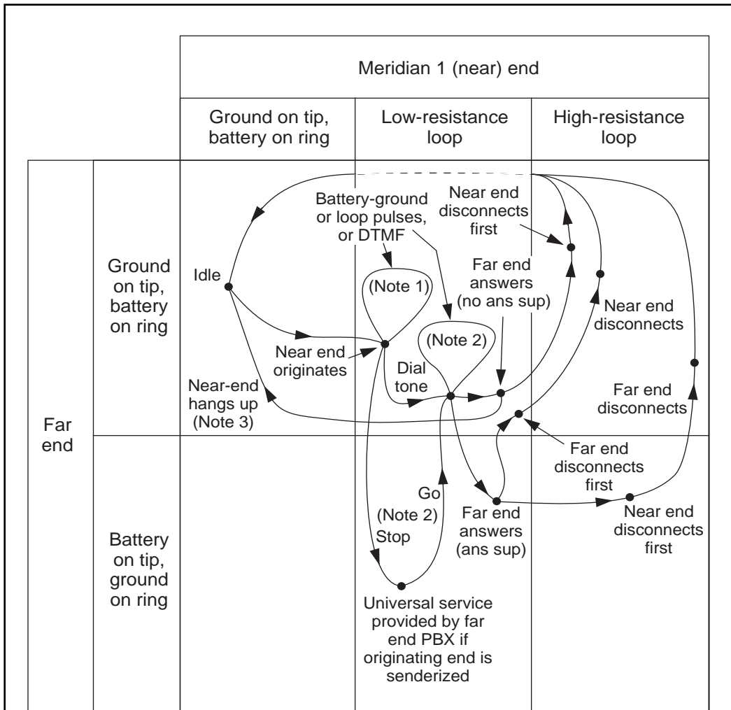
Figure 47 Two-way, Loop DR, TIE trunk call states – outgoing call through far-end PBX to CO/FEX/WATS
