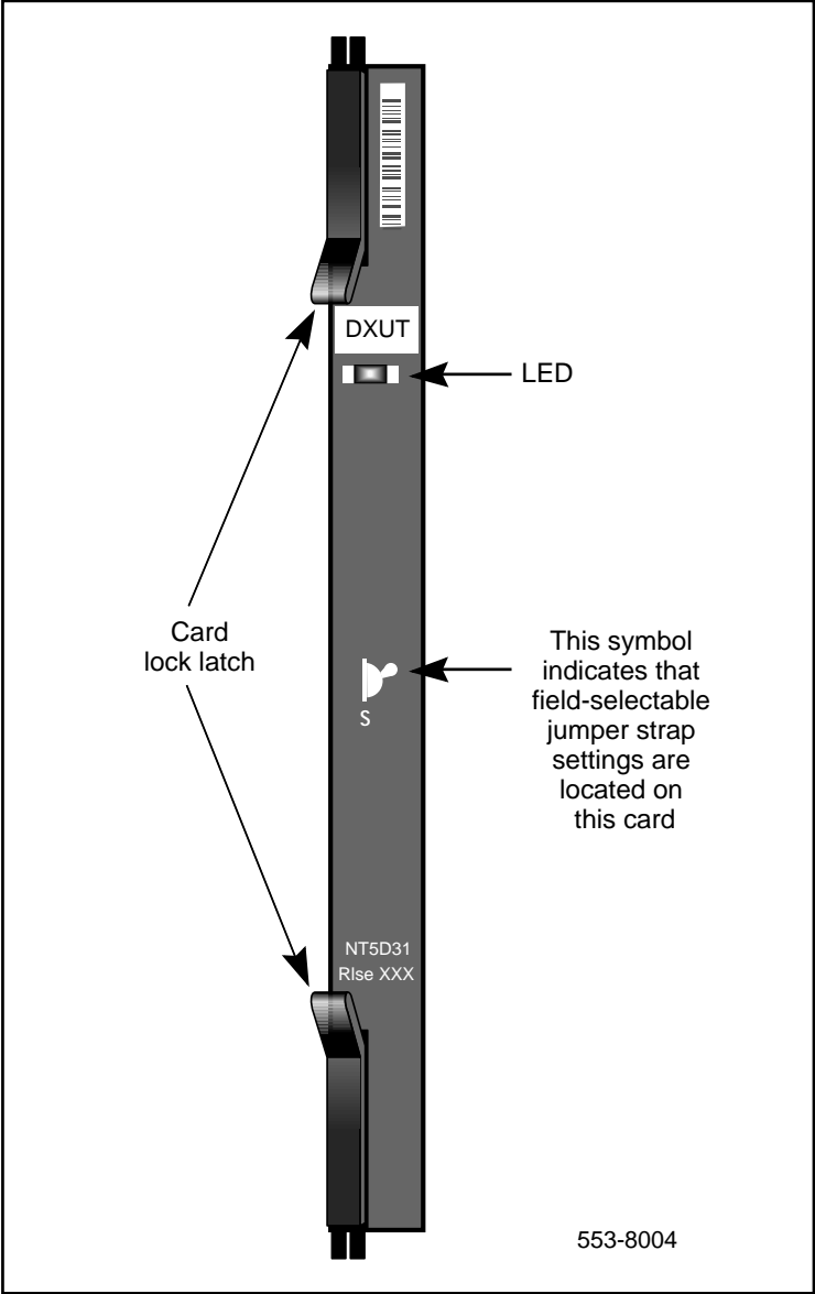
Figure 28 NT5D31 DXUT card - faceplate
