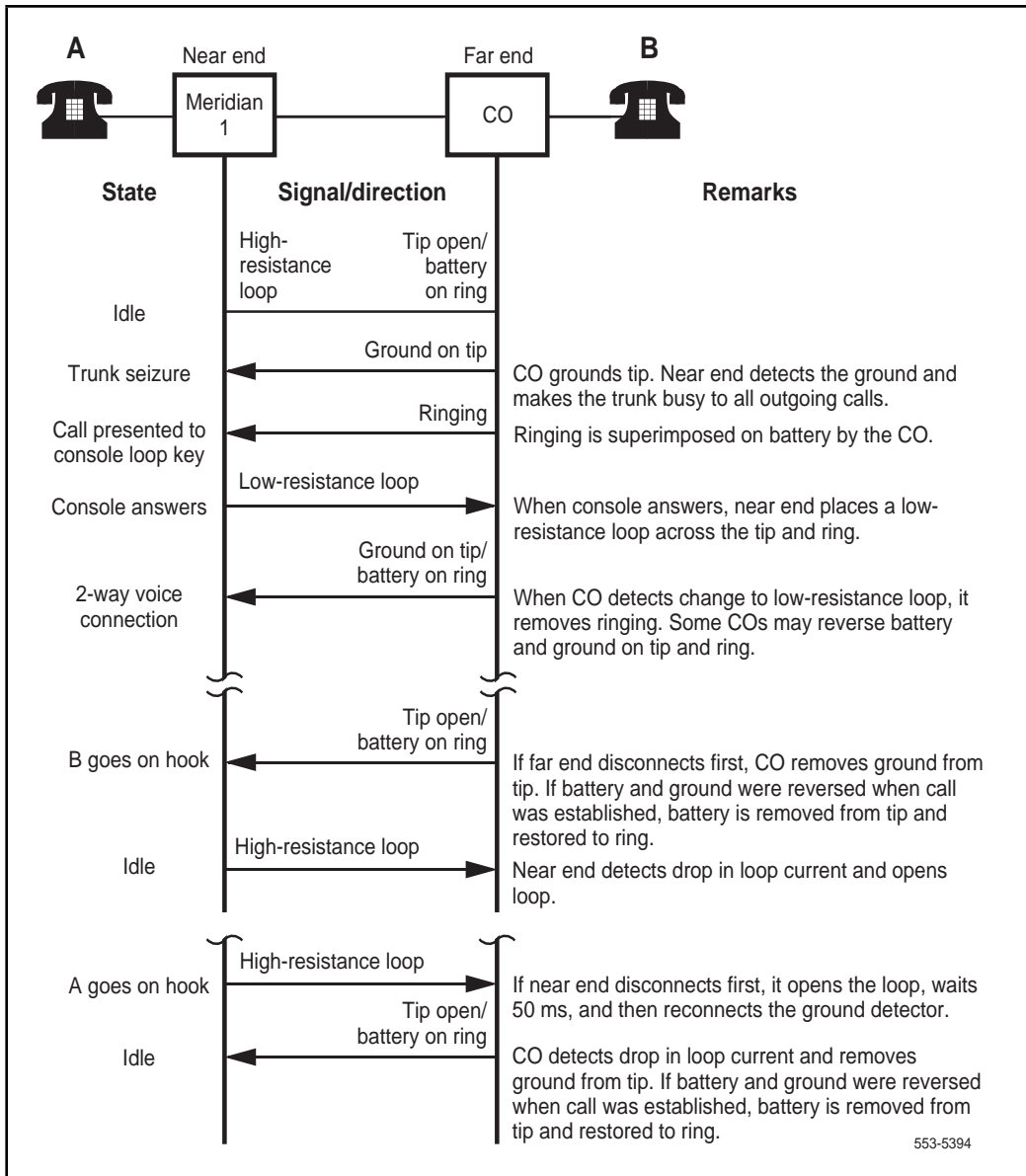
Figure 37 Ground start call connection sequence – incoming call from CO/FEX/WATS
