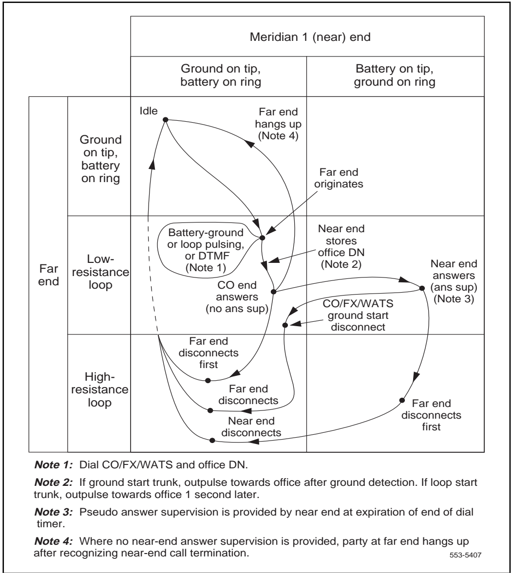
Figure 46 Two-way, Loop DR, TIE trunk call states – incoming call through senderized, tandem PBX from a CO/FEX/WATS trunk
