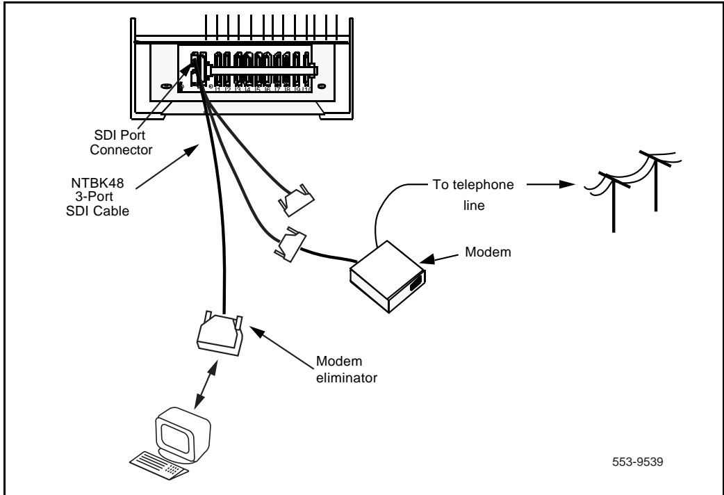
Figure 7 Option 11C site connections
