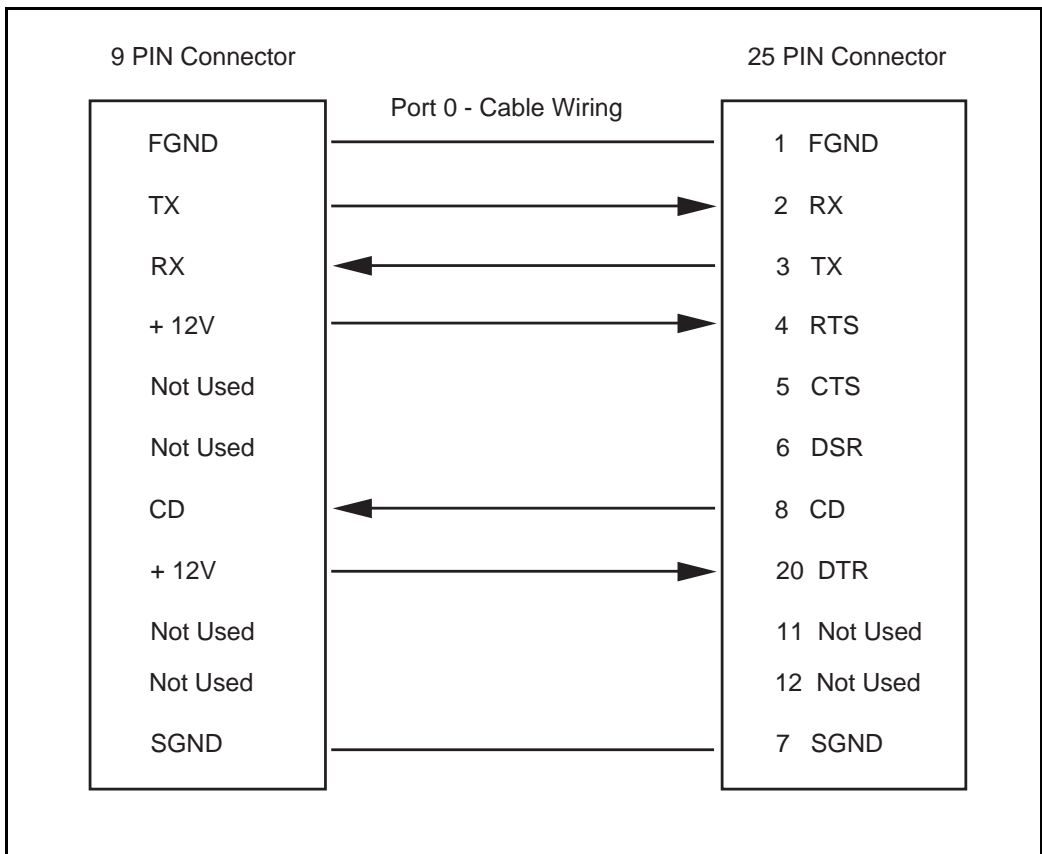
Figure 2 NTBK48 Port 0 Signal Leads
