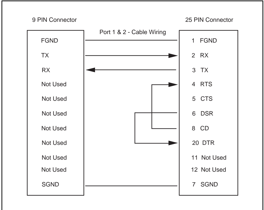
Figure 3 NTBK48 Ports 1 and 2 Signal Leads
