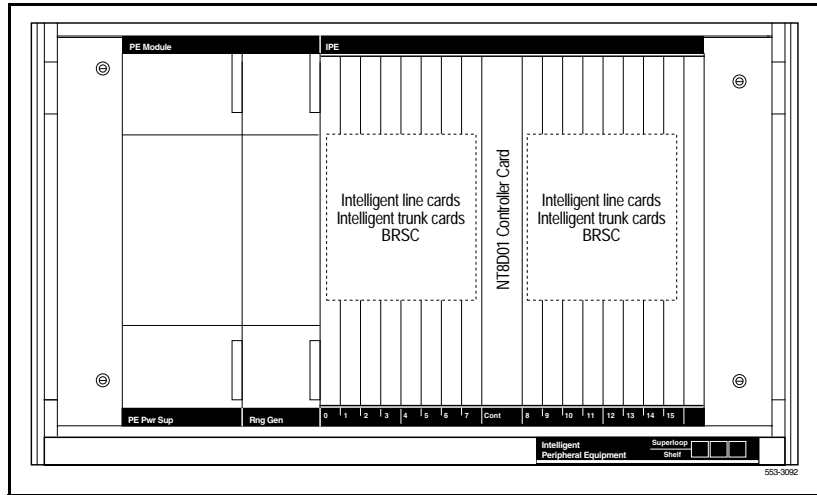
Figure 9 The NT8D37 IPE module
