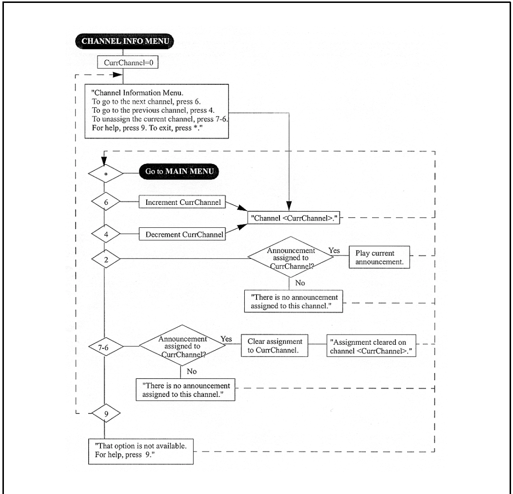
Figure 107 TUI Channel Information menu flowchart
