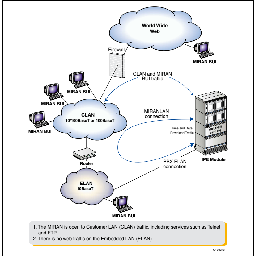
Figure 14 C-LAN connection
