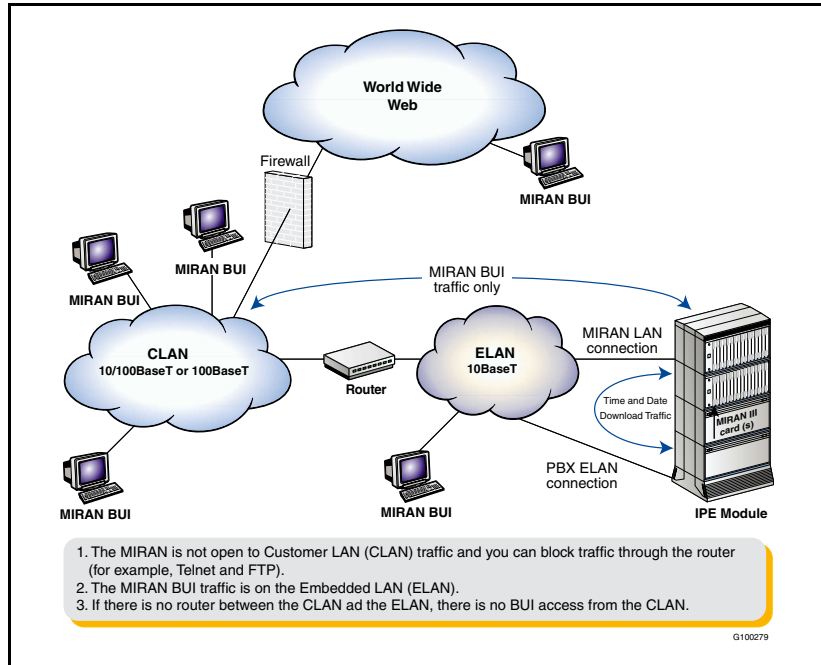
Figure 15 E-LAN Connection
