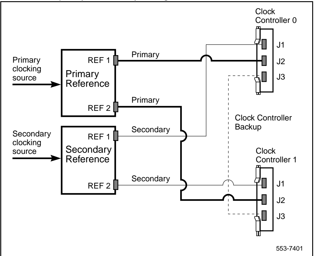
Figure 16 Clock controller, primary and secondary tracking
