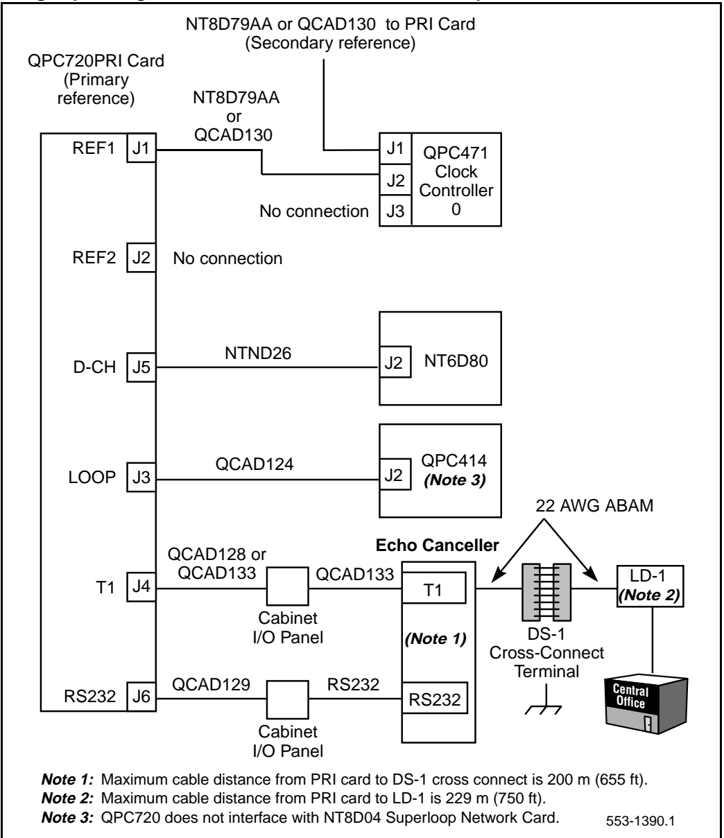
Figure 58 Half group cabling with echo canceller, for the QPC720 on Options 51C and 61C
