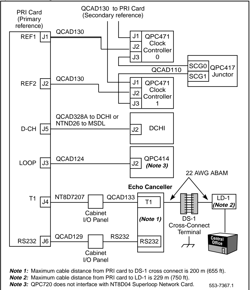
Figure 62 Option 81C cabling for the QPC720 with echo canceller
