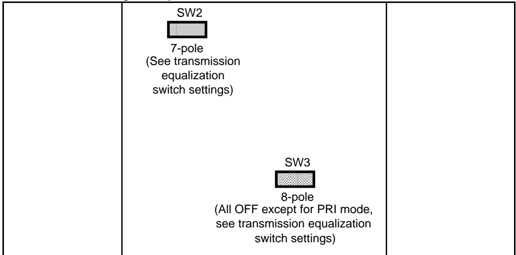
Figure 64 QPC720 switch settings for Options 51C and 61C
