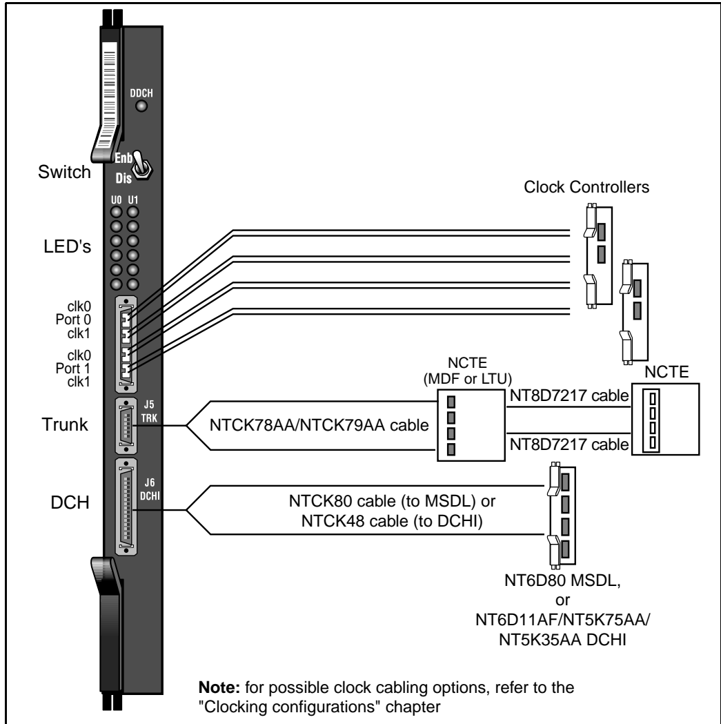
Figure 29 DDP2 cable for Meridian 1 systems with an I/O panel
