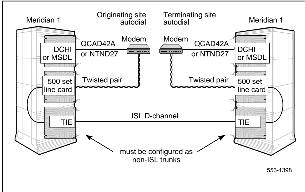
Figure 81 ISL in shared mode
