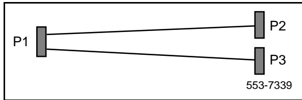
Figure 9 120 Ohm Dual PRI to I/O Panel cable (8ft).
