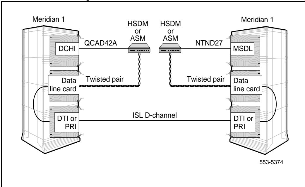
Figure 85 ISL dedicated mode: using PRI/DTI trunk
