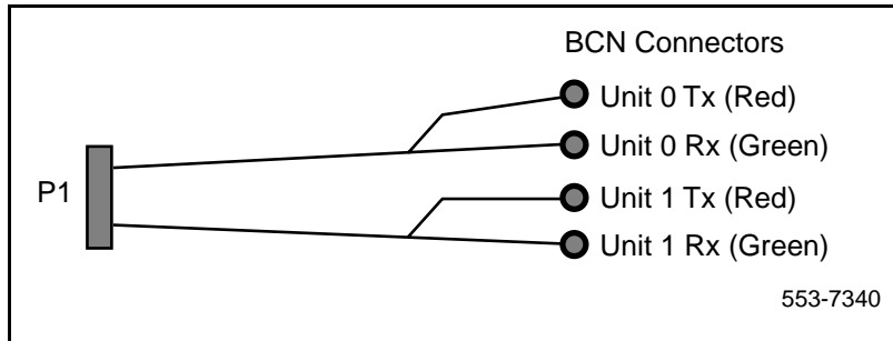
Figure 11 75 Ohm Dual PRI Coax Cable (40ft).
