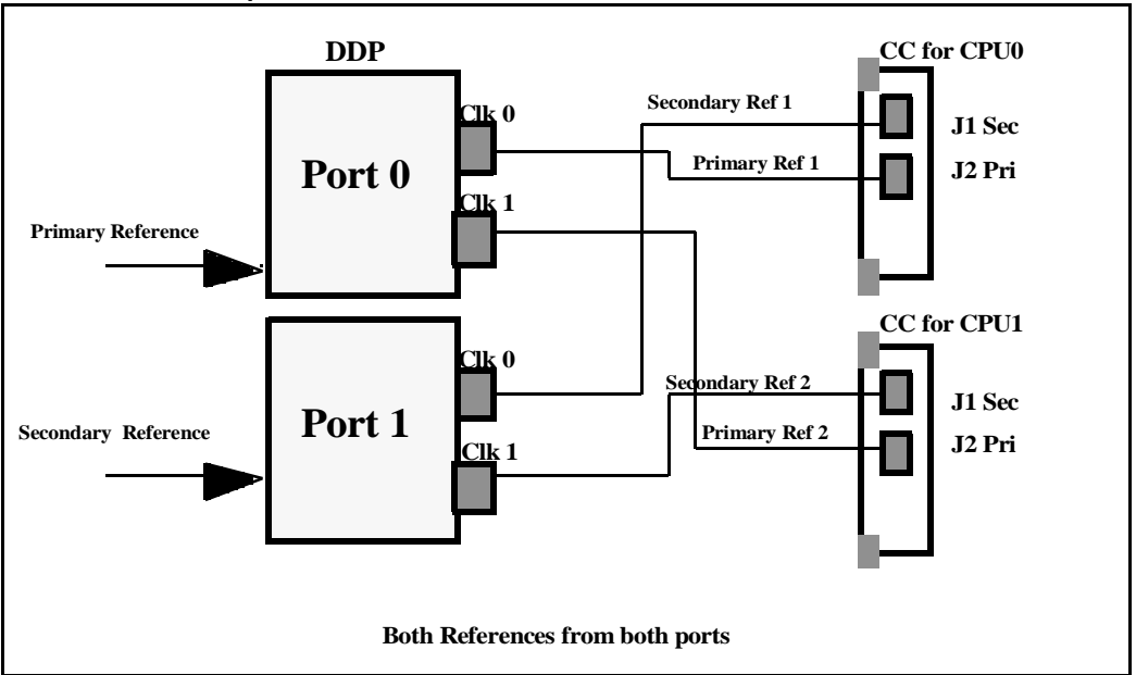
Figure 44 Clock Controller - Option 4
