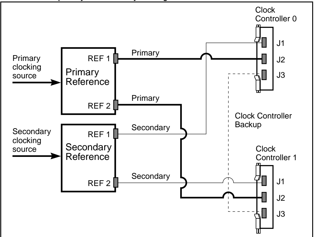
Figure 31 Clock Controller primary and secondary tracking
