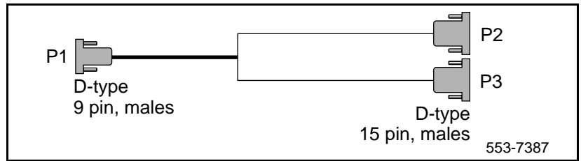
Figure 27 NTCK46AA/AB/AC/AD
