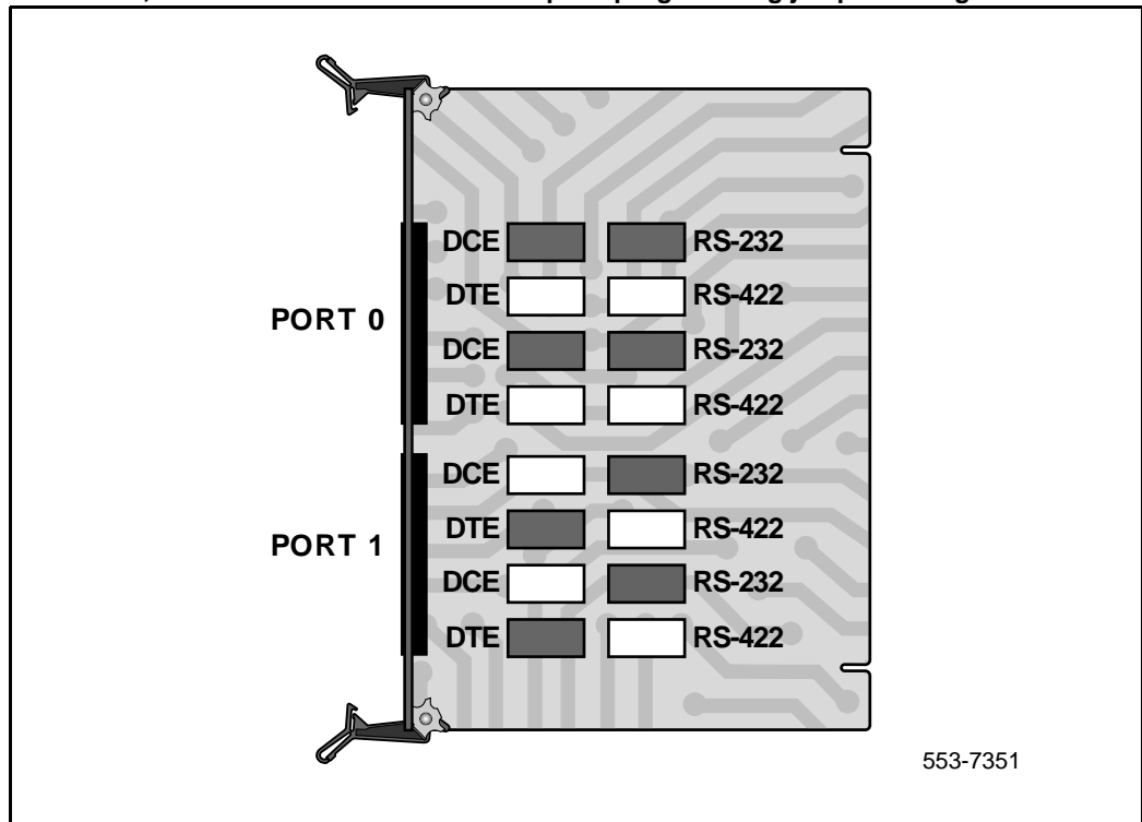
Figure 79 NT6D11AB, NT6D11AD DCHI with ISL low-speed programming jumper settings
