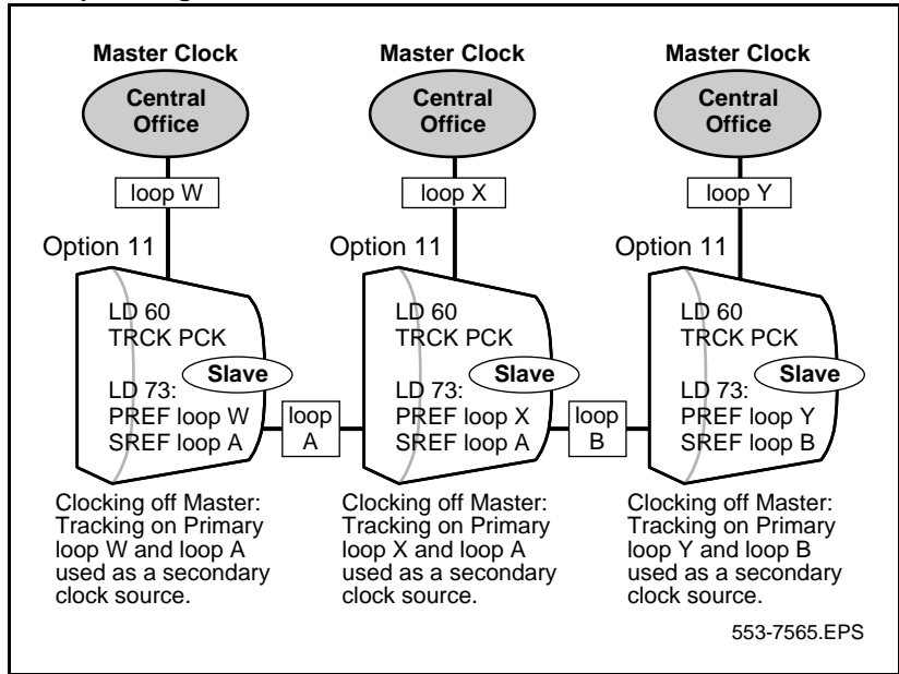
Figure 75 Example 5, digital connection to the CO
