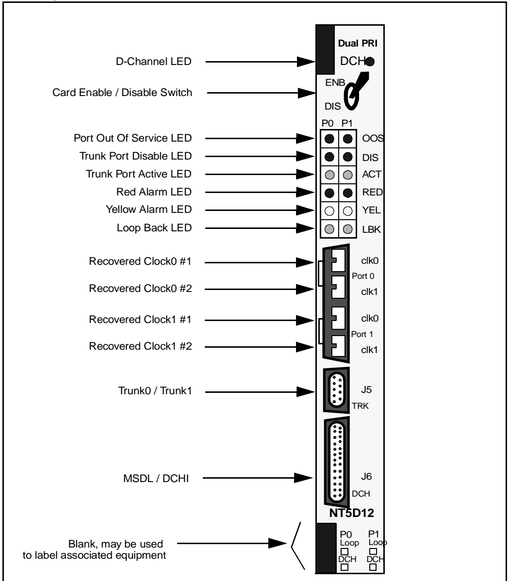
Figure 37 DDP faceplate - detailed view
