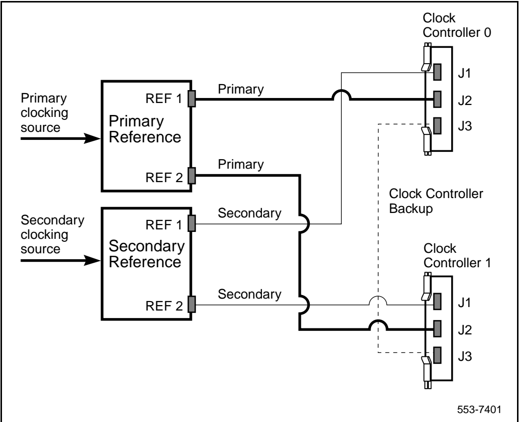
Figure 40 Clock Controller primary and secondary tracking
