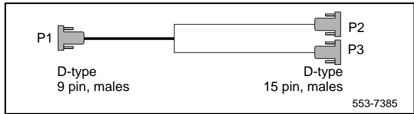
Figure 24 NTCK78AA
