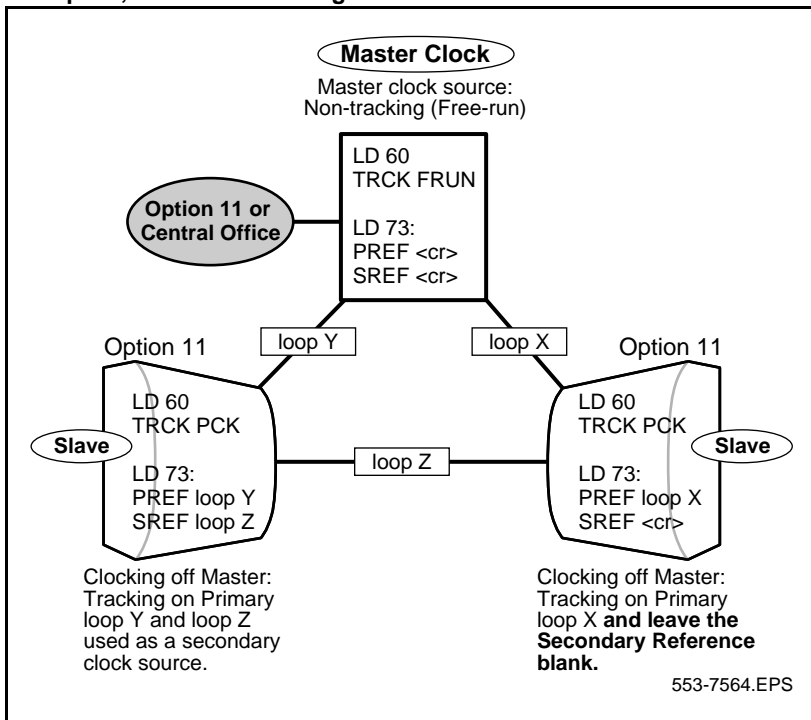
Figure 74 Example 4, Alternate Clocking from the same CO
