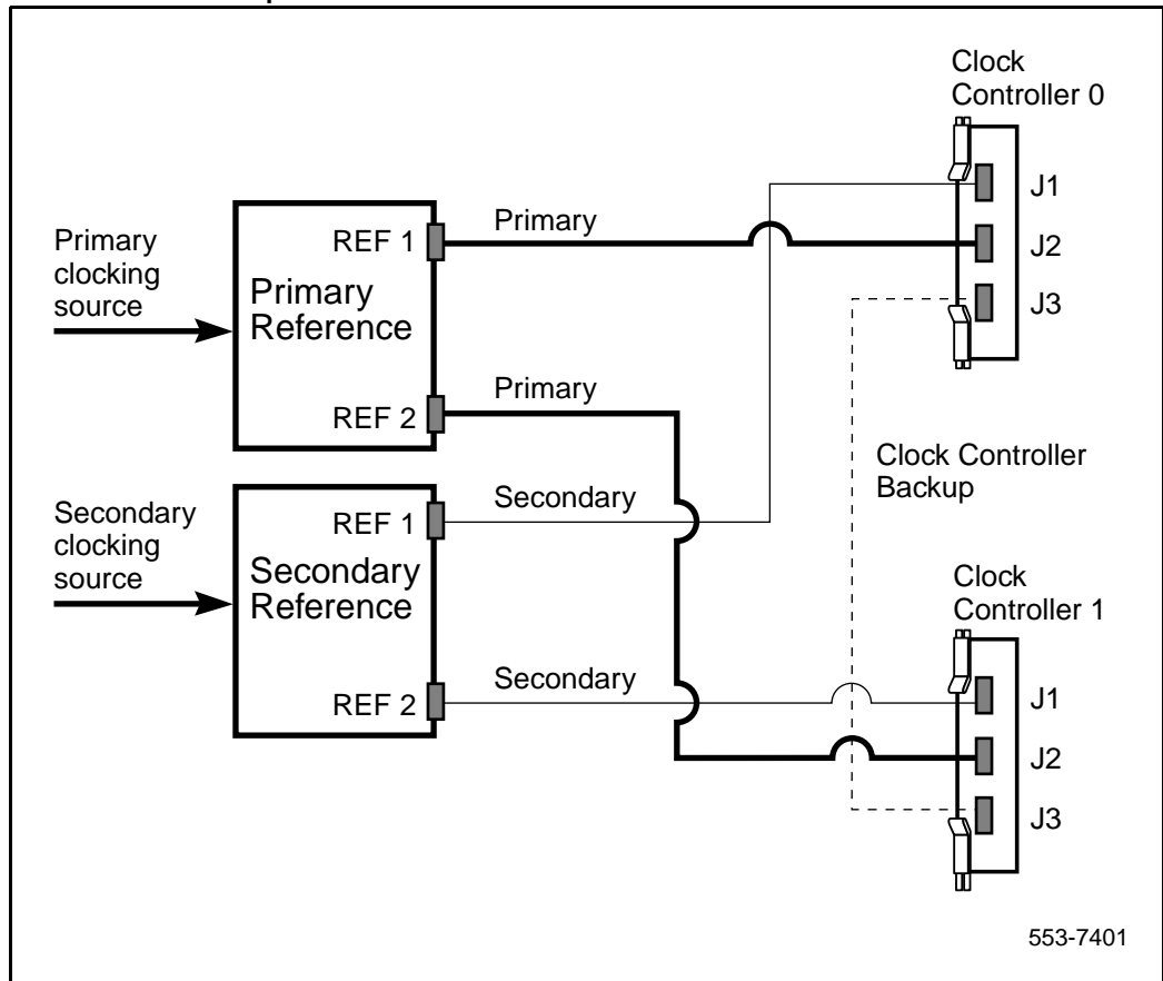
Figure 32 Clock Controller – Option 1
