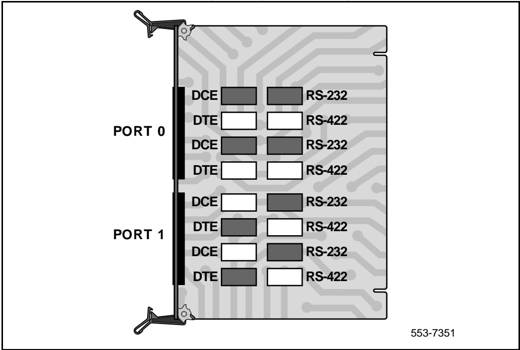
Figure 47 NT6D11 DCH with ISL low-speed programming jumper settings
