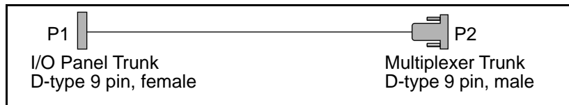
Figure 23 NT8D7217
