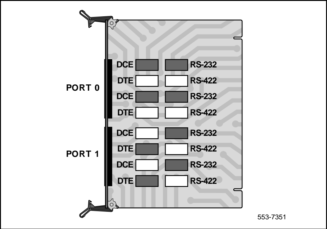
Figure 49 QPC757 option and PRI/ISL low speed programming switch settings
