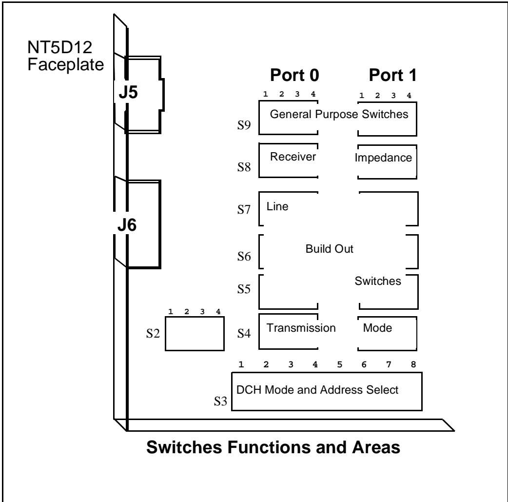
Figure 68 Switch functional areas on the NT5D12
