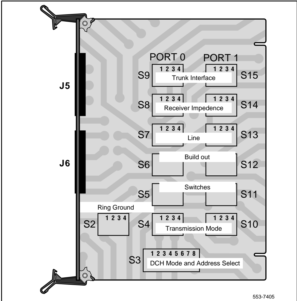
Figure 66 Switch functional areas
