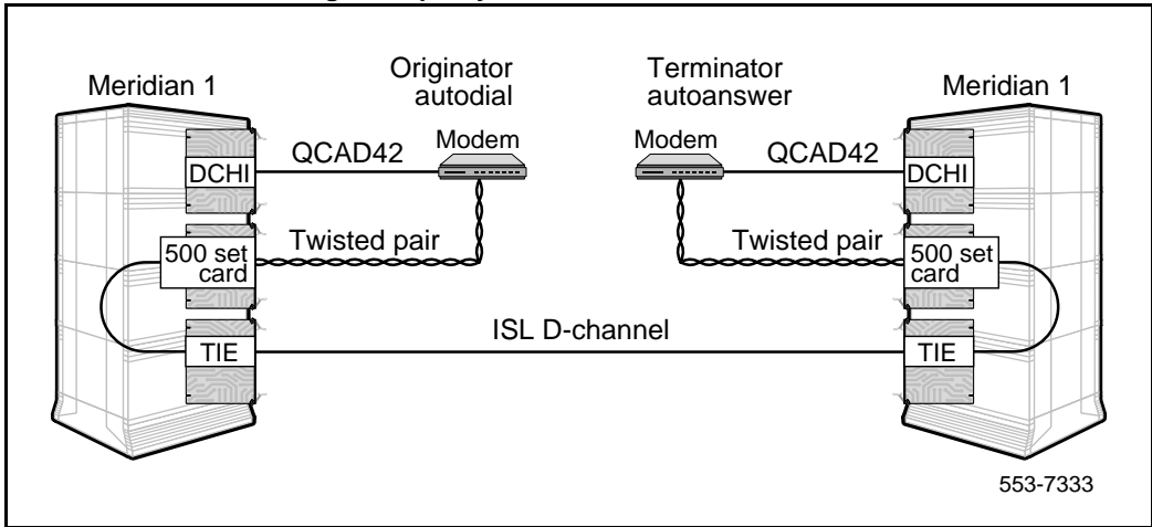
Figure 83 ISL dedicated mode: using dial-up Hayes Smartmodem 2400
