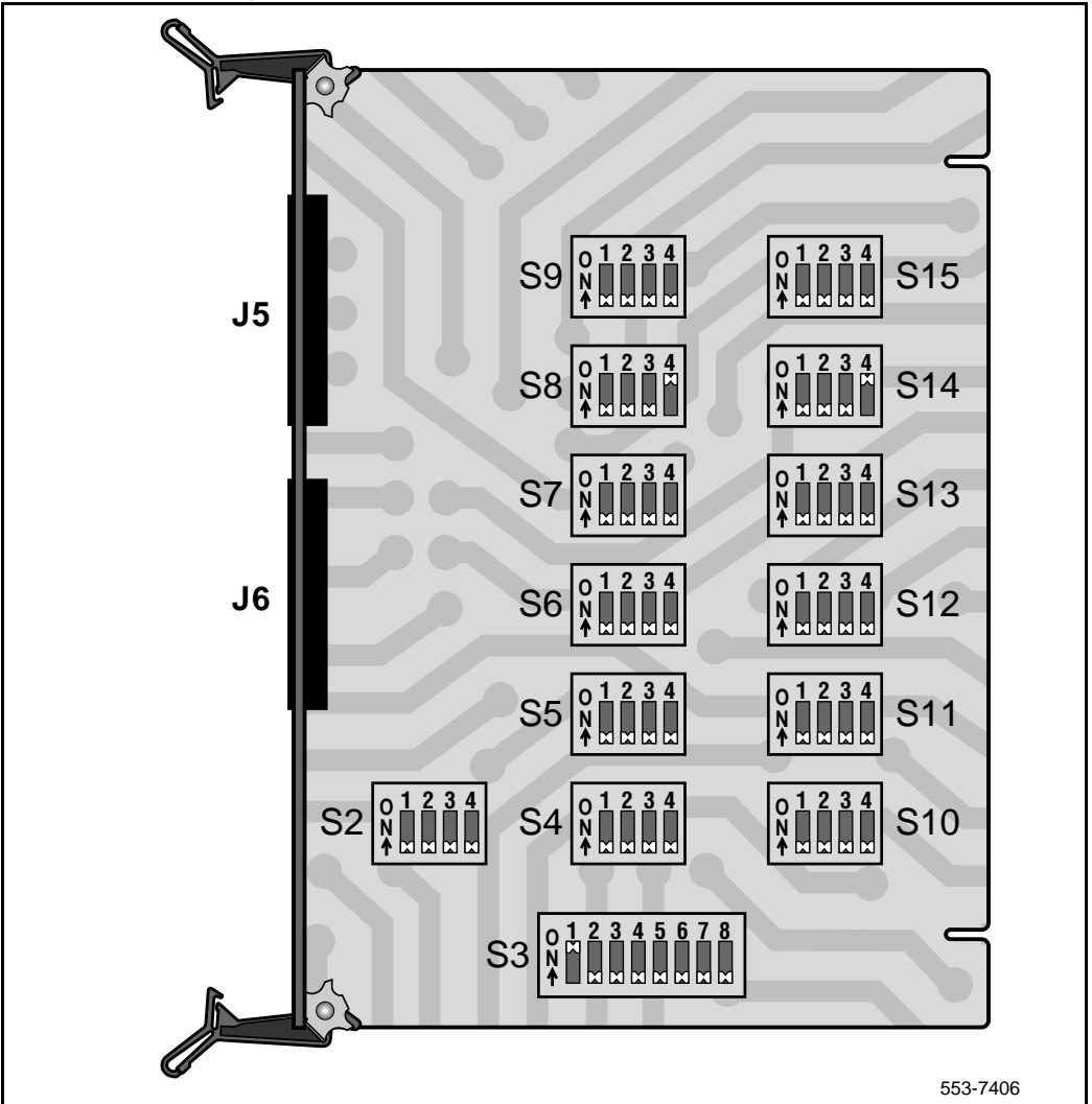
Figure 67 Switch default settings
