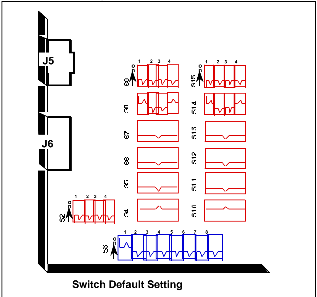
Figure 69 NT5D12 switch default settings
