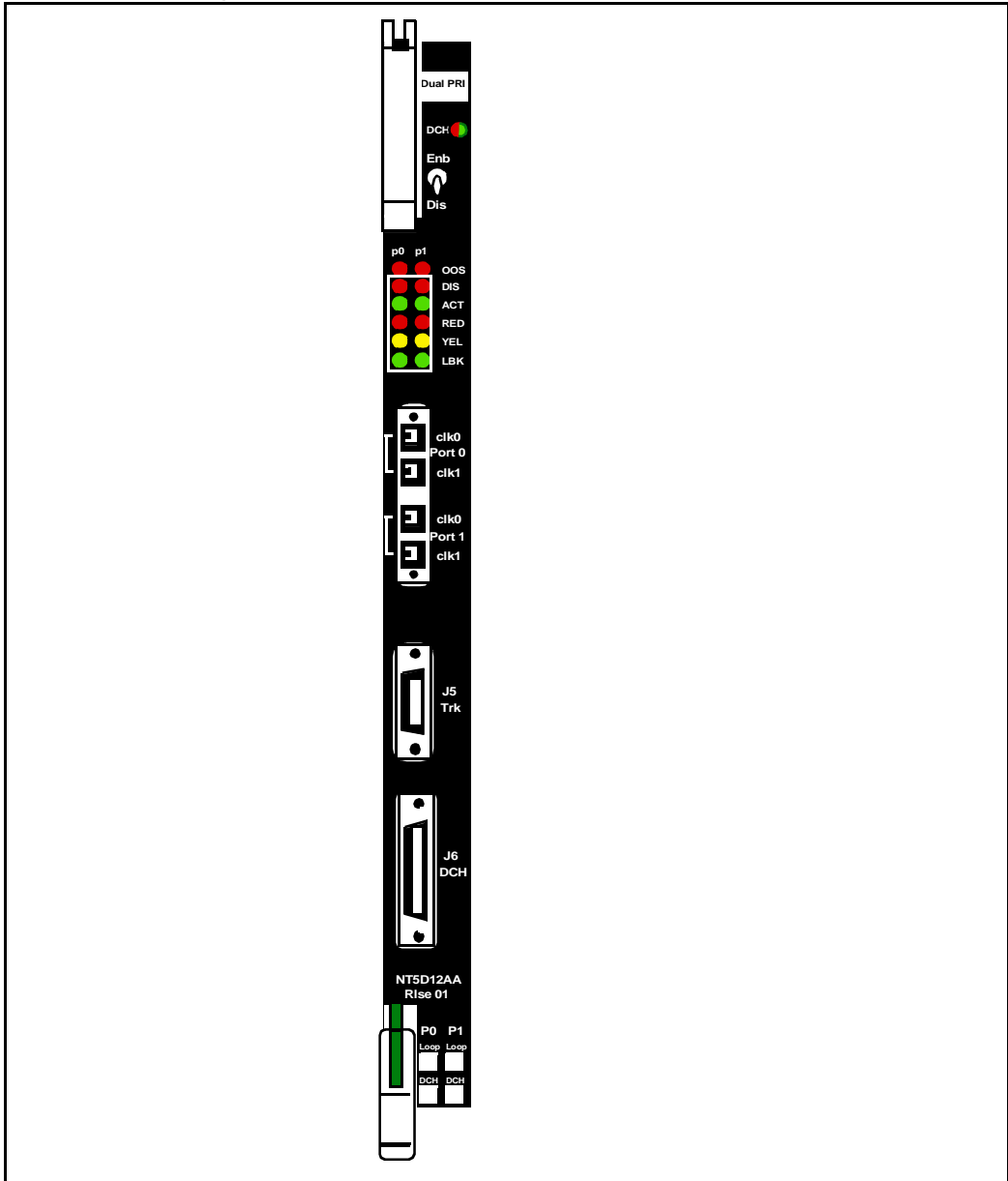
Figure 36 NT5D12 faceplate - general view
