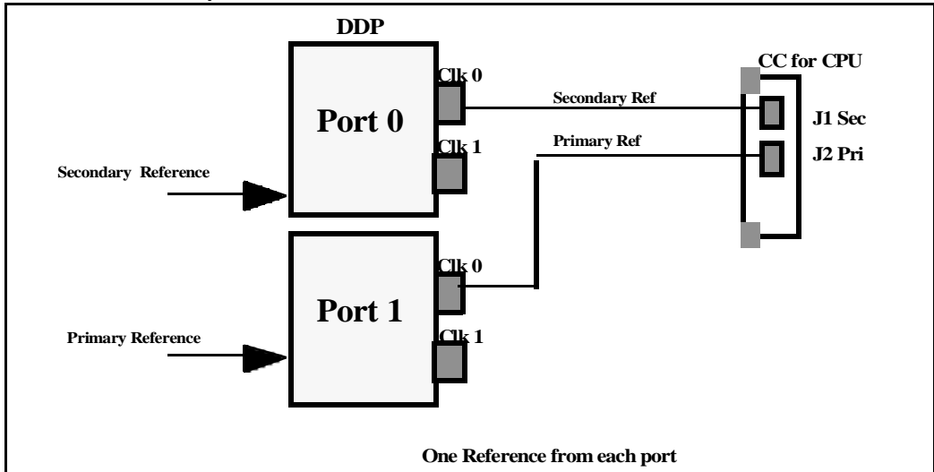
Figure 41 Clock Controller - Option 1
