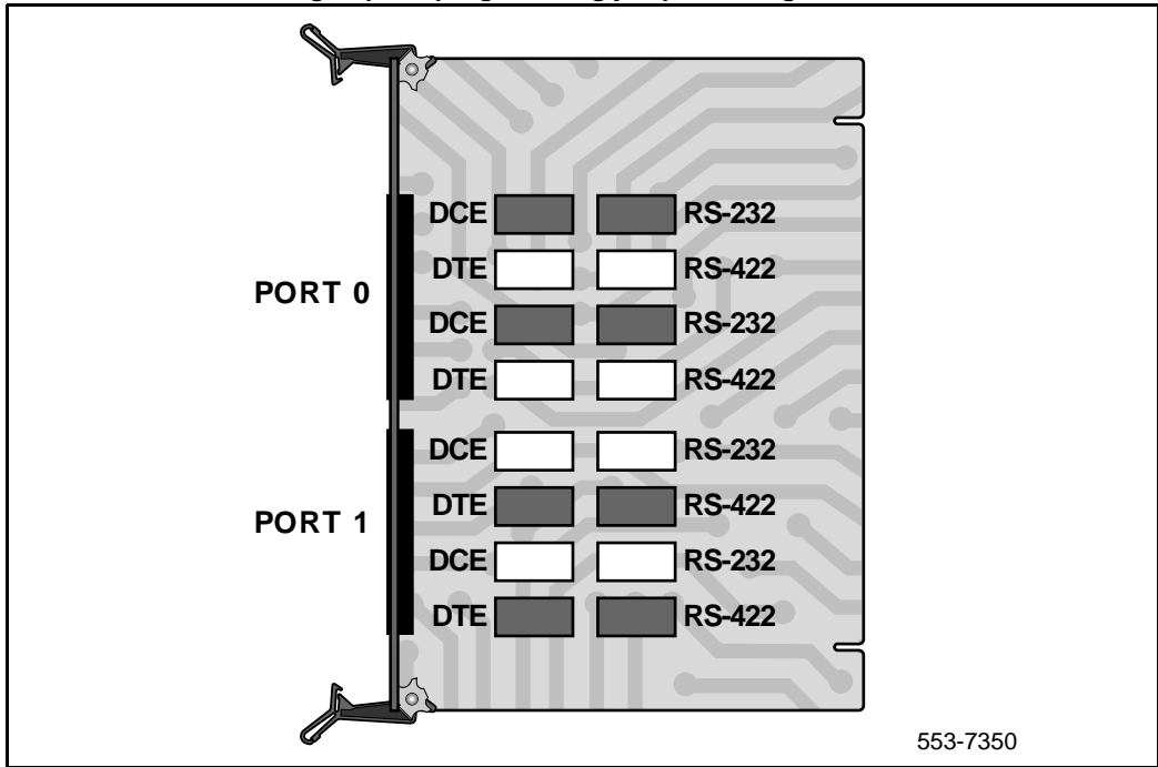
Figure 46 NT6D11 DCH with ISL high-speed programming jumper settings
