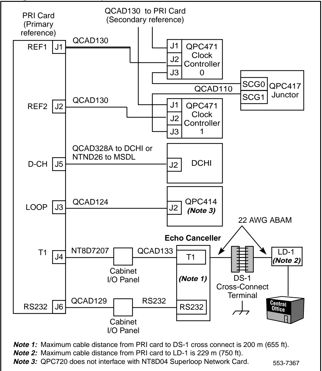
Figure 56 Cabling for the NT8D72 on Option 81C with echo canceller
