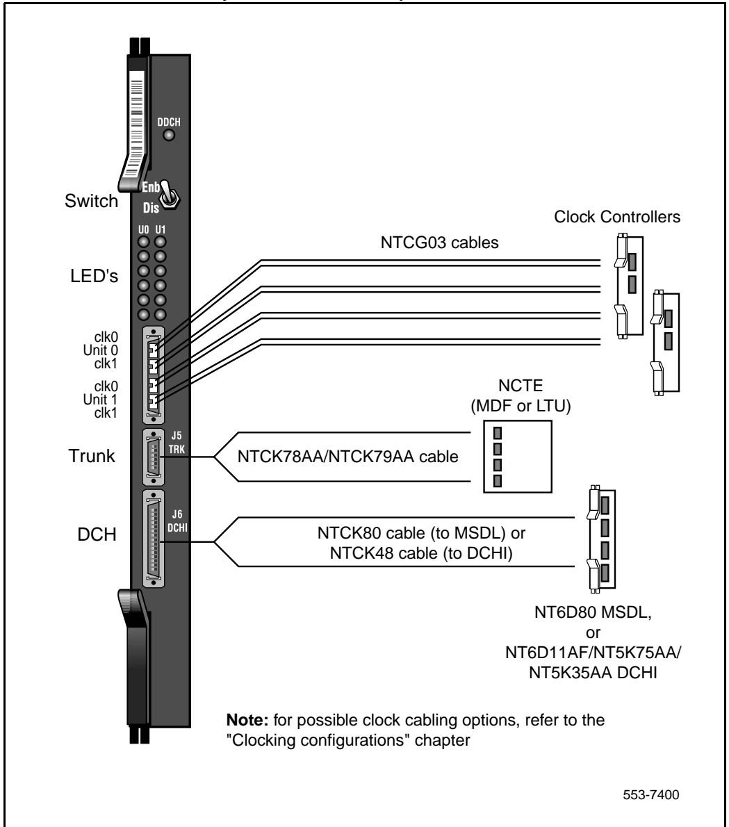
Figure 30 DDP2 cable for Meridian 1 systems without an I/O panel
