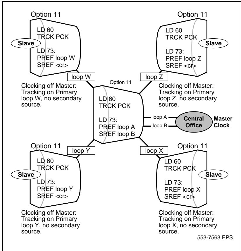
Figure 73 Example 3, Clocking Hierarchy referenced to a Public Network Master Clock
