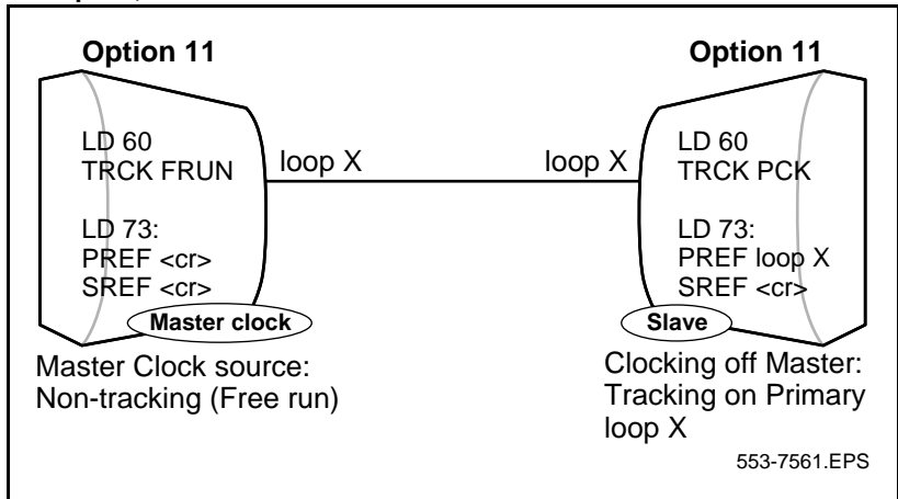
Figure 71 Example 1, Isolated Private Network
