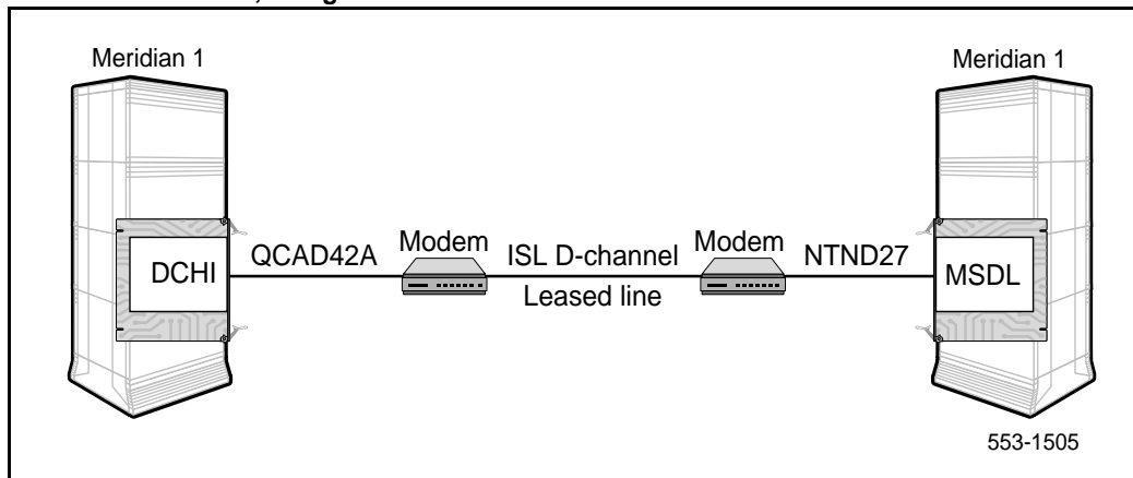
Figure 82 ISL dedicated mode, using leased line
