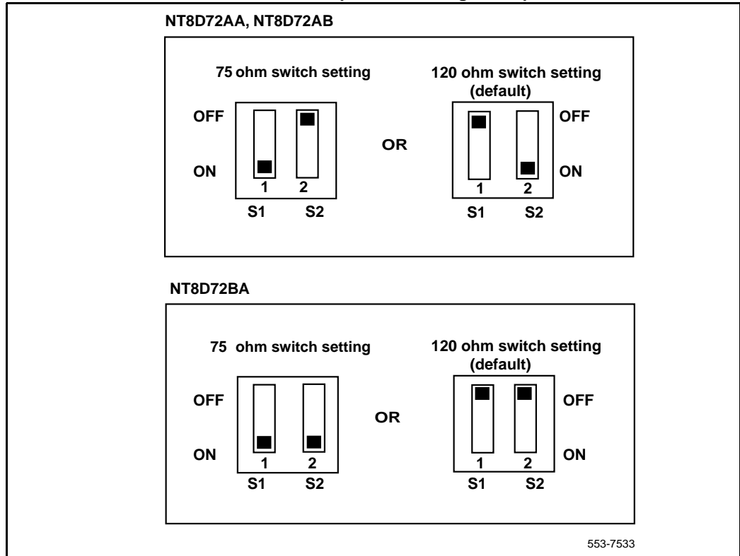
Figure 63 NT8D72AA, NT8D72AB, NT8D72BA PRI dip switch settings for Options 51C, 61C and 81C
