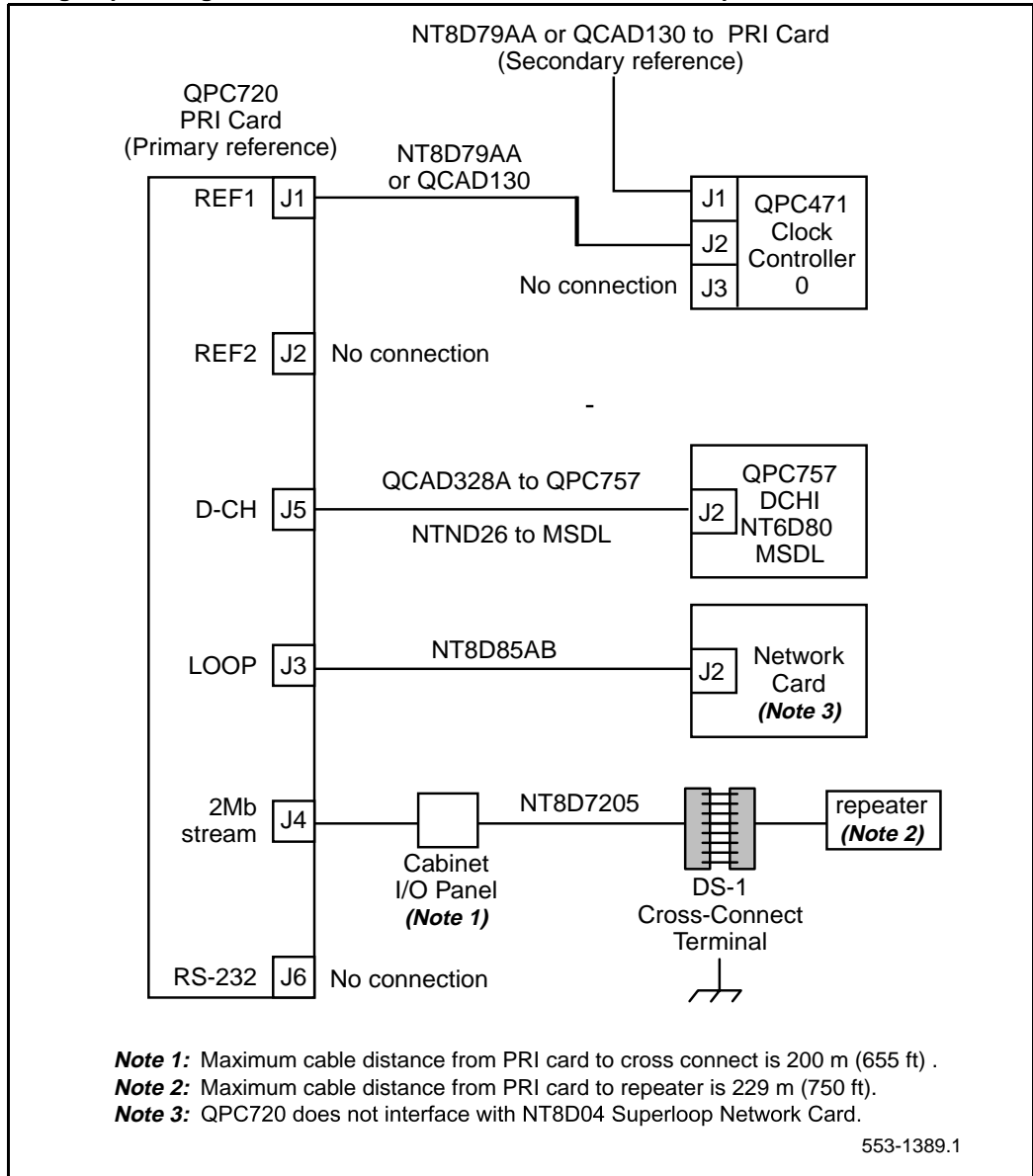
Figure 57 Half group cabling without echo canceller, for the QPC720 on Options 51C and 61C
