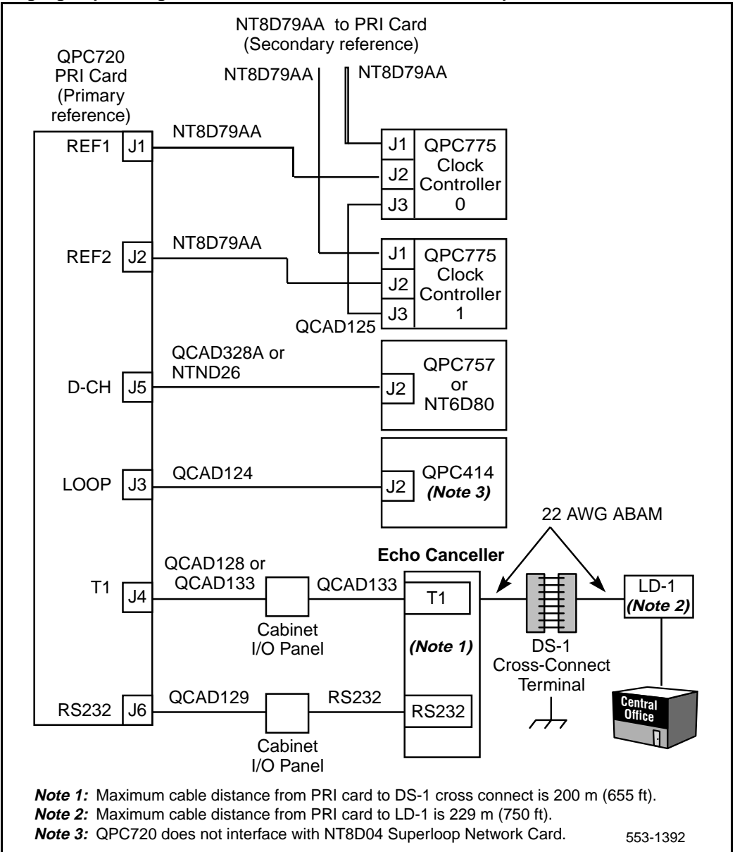
Figure 60 Single group cabling with echo canceller, for the QPC720 on Options 51C and 61C
