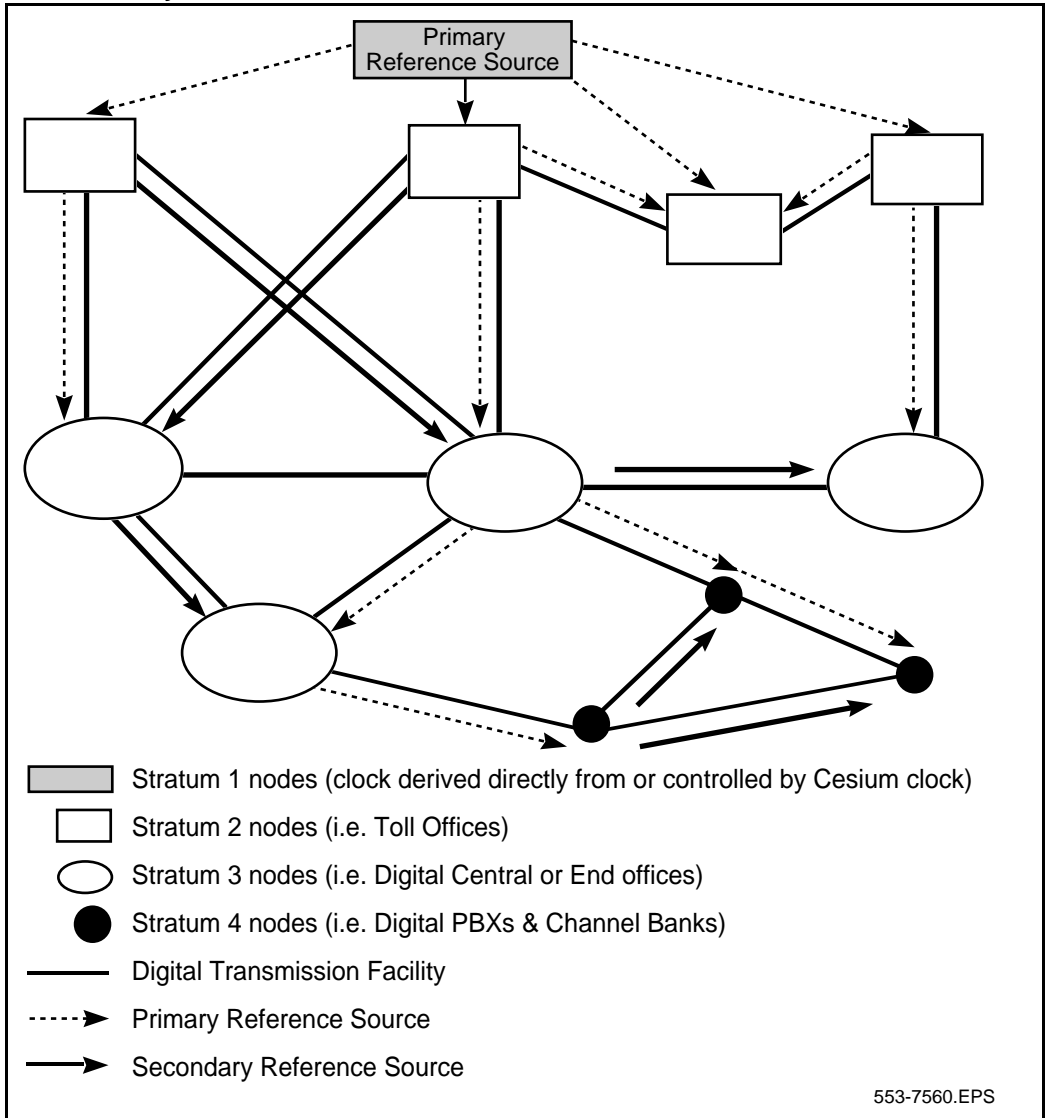
Figure 70 Hierarchical Synchronization
