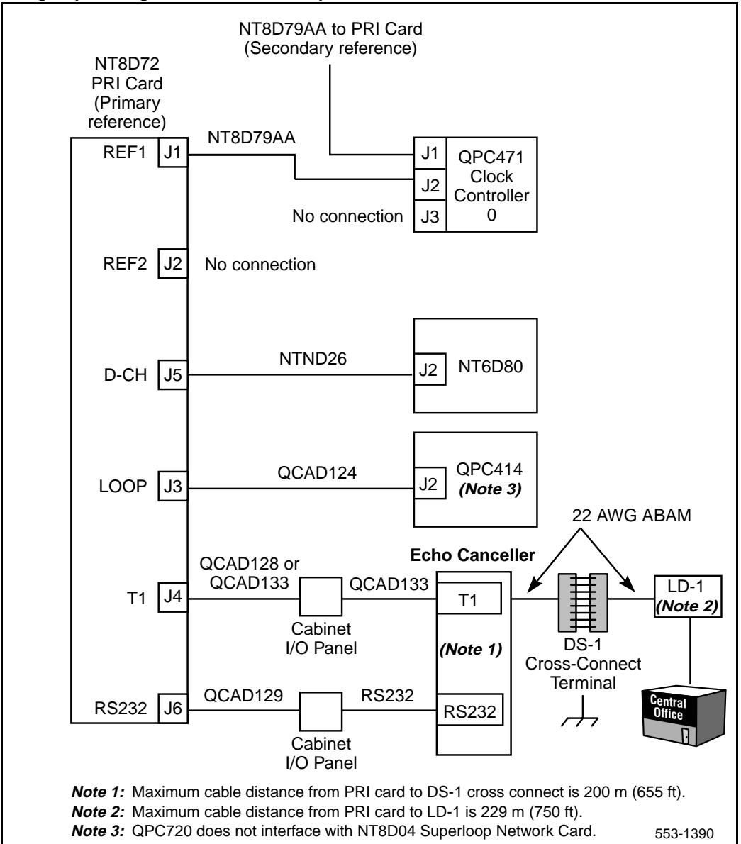
Figure 52 Half group cabling for the NT8D72 on Options 51C and 61C, with echo canceller
