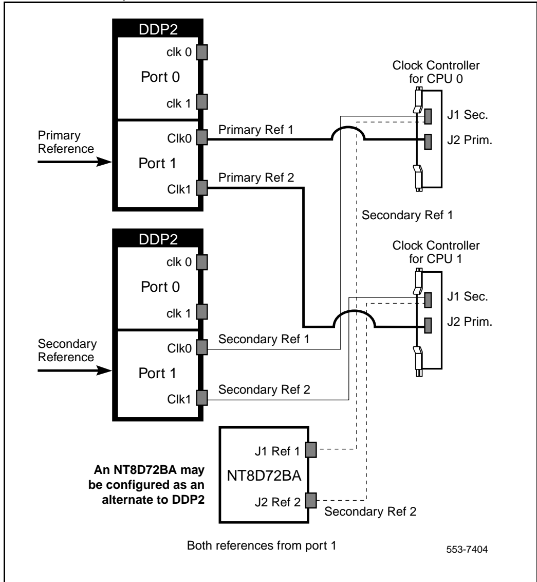
Figure 34 Clock Controller – Option 3
