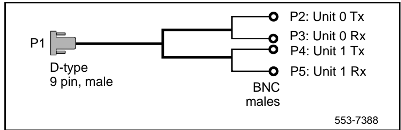
Figure 25 NTCK79AA
