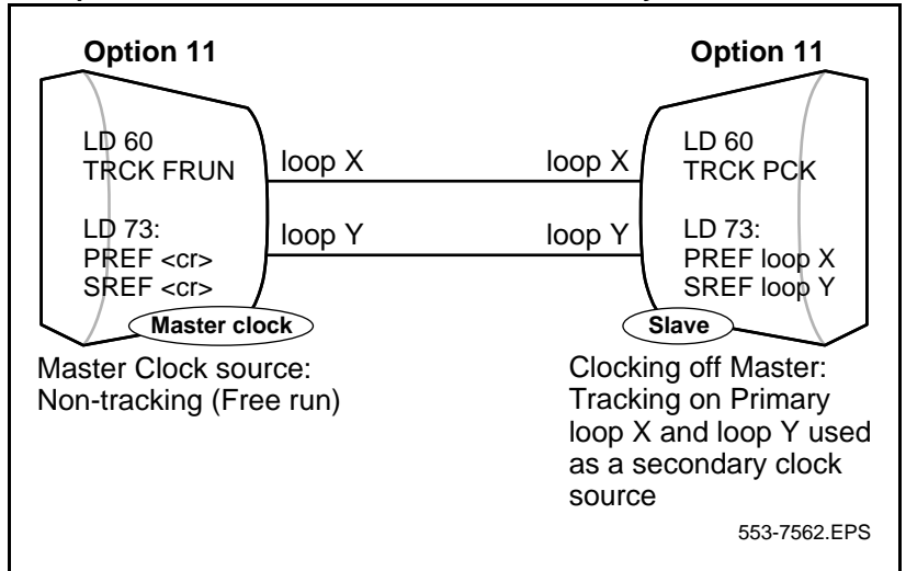
Figure 72 Example 2, Isolated Private Network with Secondary Reference Clock
