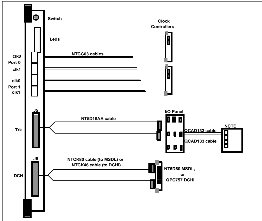
Figure 39 DDP cable for Meridian 1 systems with an I/O panel
