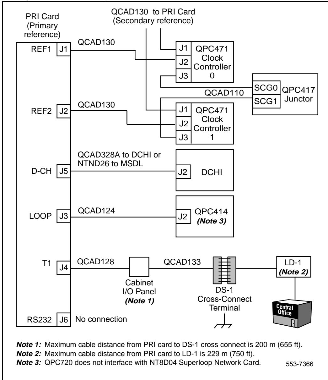
Figure 55 Cabling for the NT8D72 on Option 81C without echo canceller
