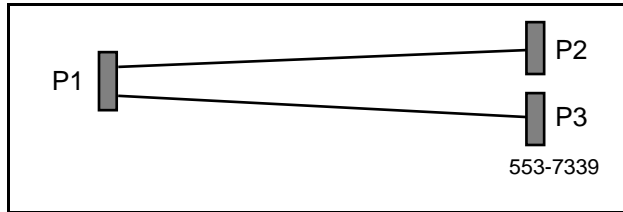
Figure 14 Dual PRI to Clock Controller cable (10ft)
