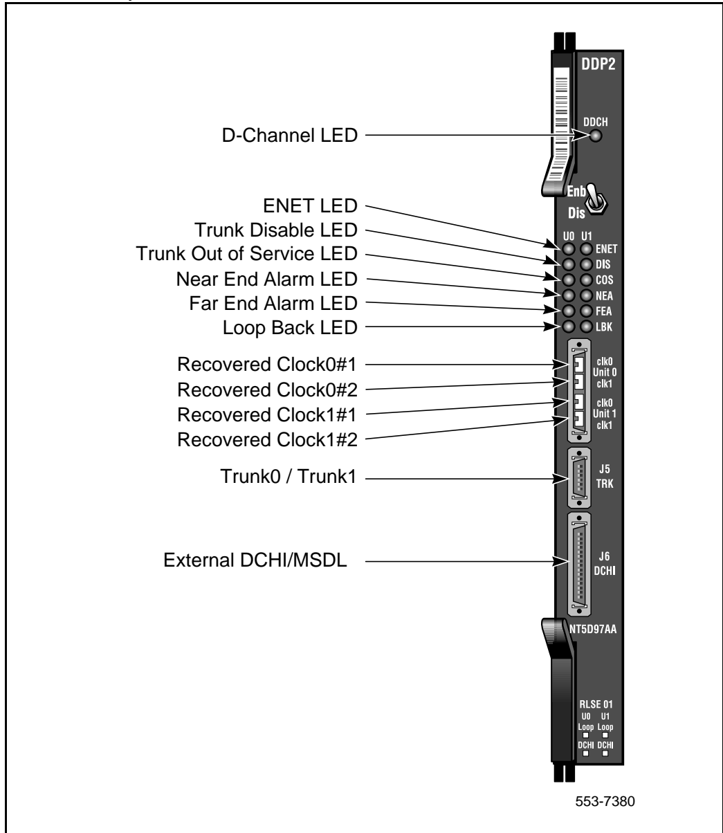
Figure 21 NT5D97AA faceplate
