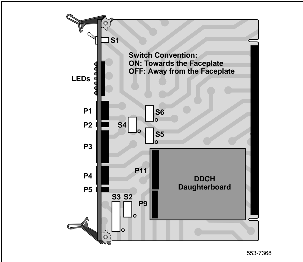
Figure 65 NTCK43 switch settings
