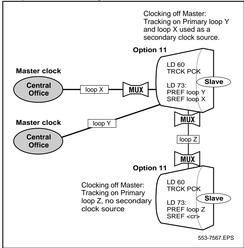
Figure 77 Example 7, Network Clocking with MUX
