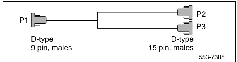
Figure 22 NTCK45AA
