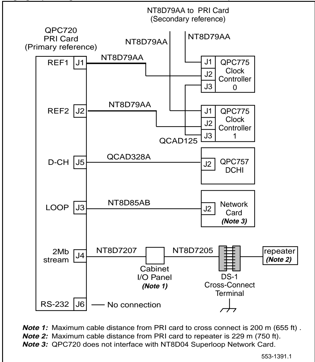
Figure 59 Single group cabling without echo canceller, for the QPC720 on Options 51C and 61C
