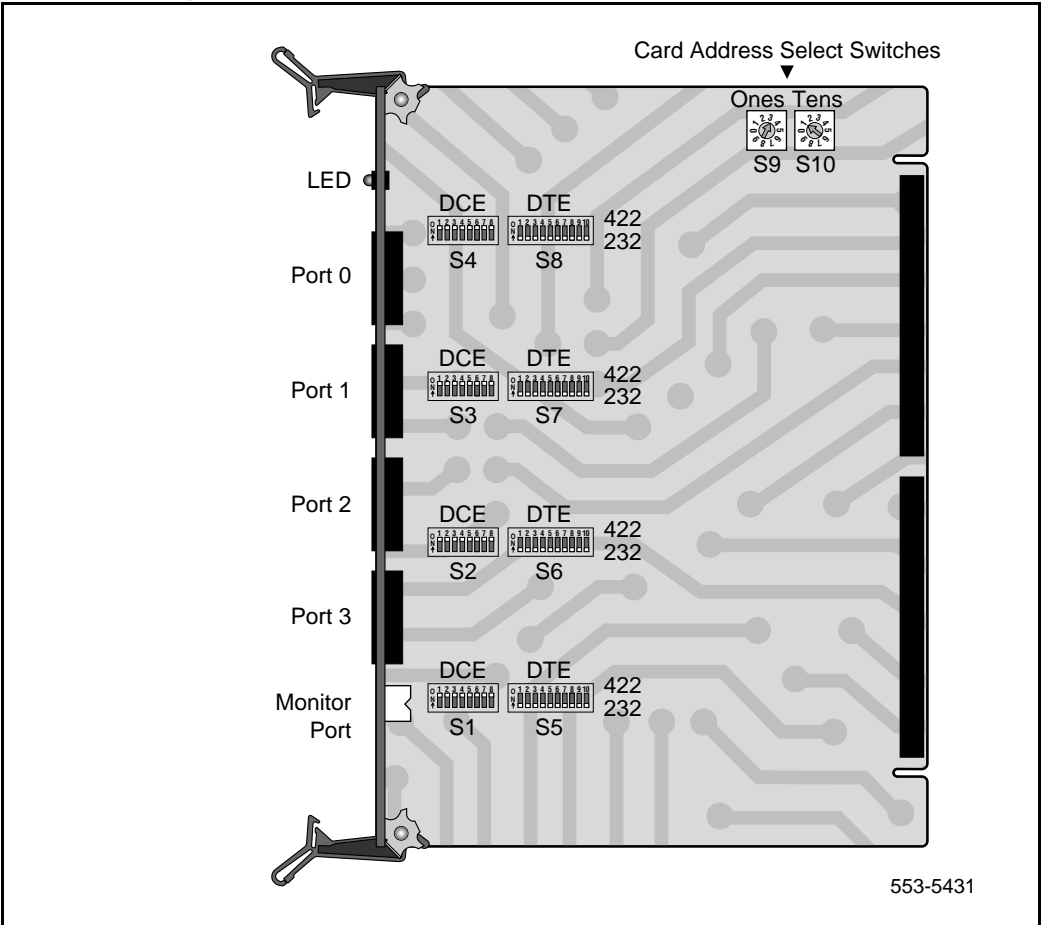
Figure 80 MSDL/ISL settings
