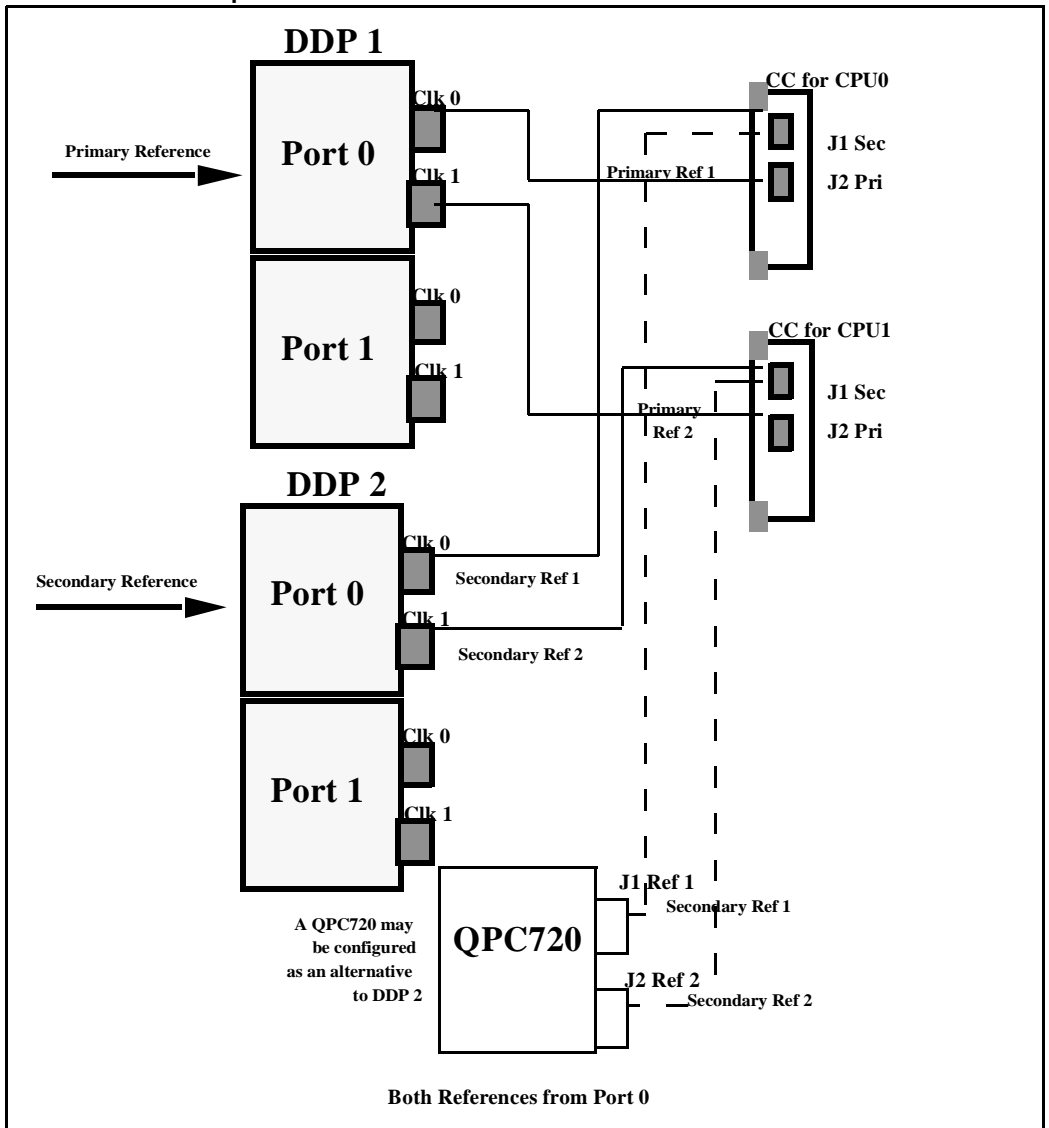
Figure 42 Clock Controller - Option 2
