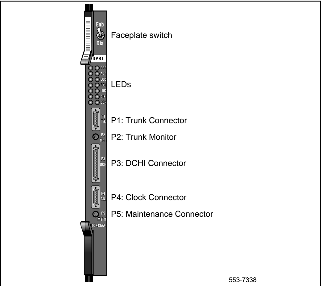
Figure 8 NTCK43 DPRI faceplate
