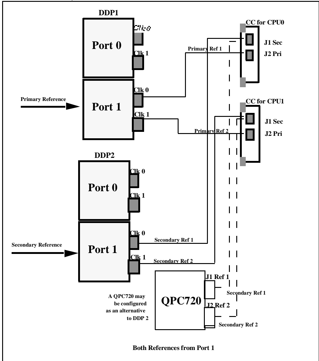
Figure 43 Clock Controller - Option 3
