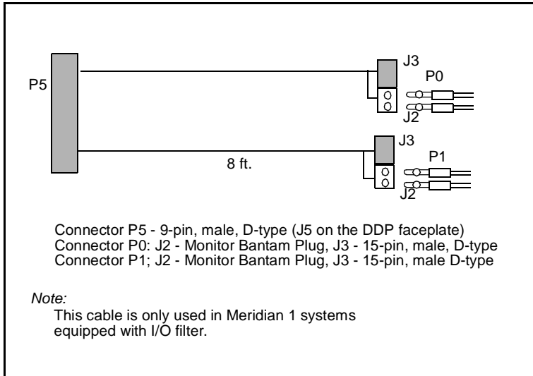
Figure 38 NT5D16AA
