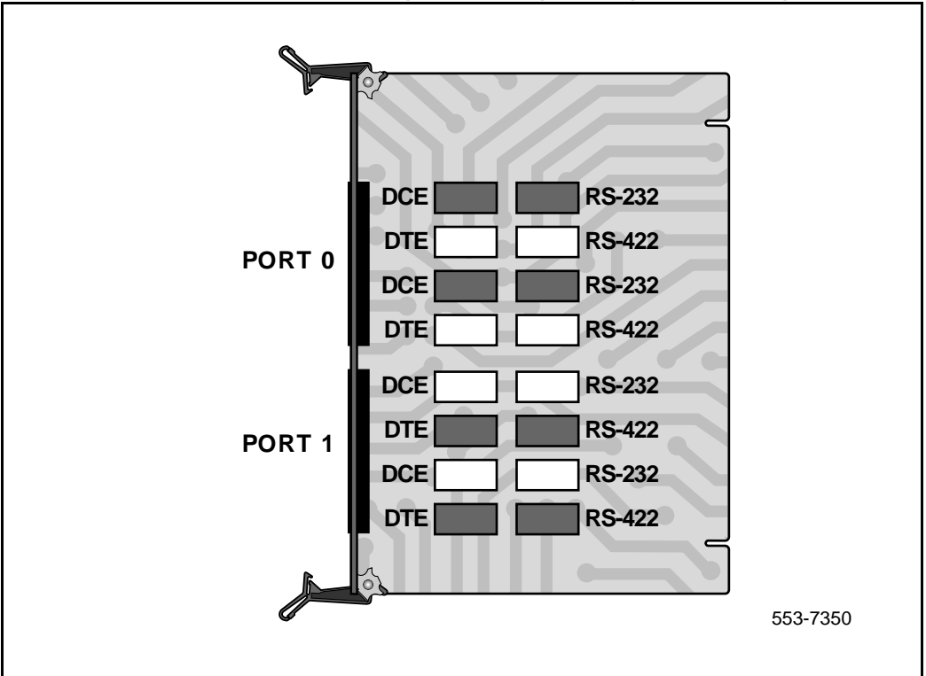
Figure 78 NT6D11AB, NT6D11AD DCHI with ISL high-speed programming jumper settings
