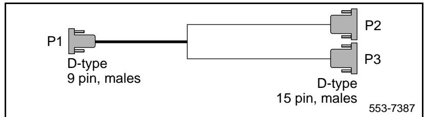
Figure 28 NTCK80AA/AB/AC/AD
