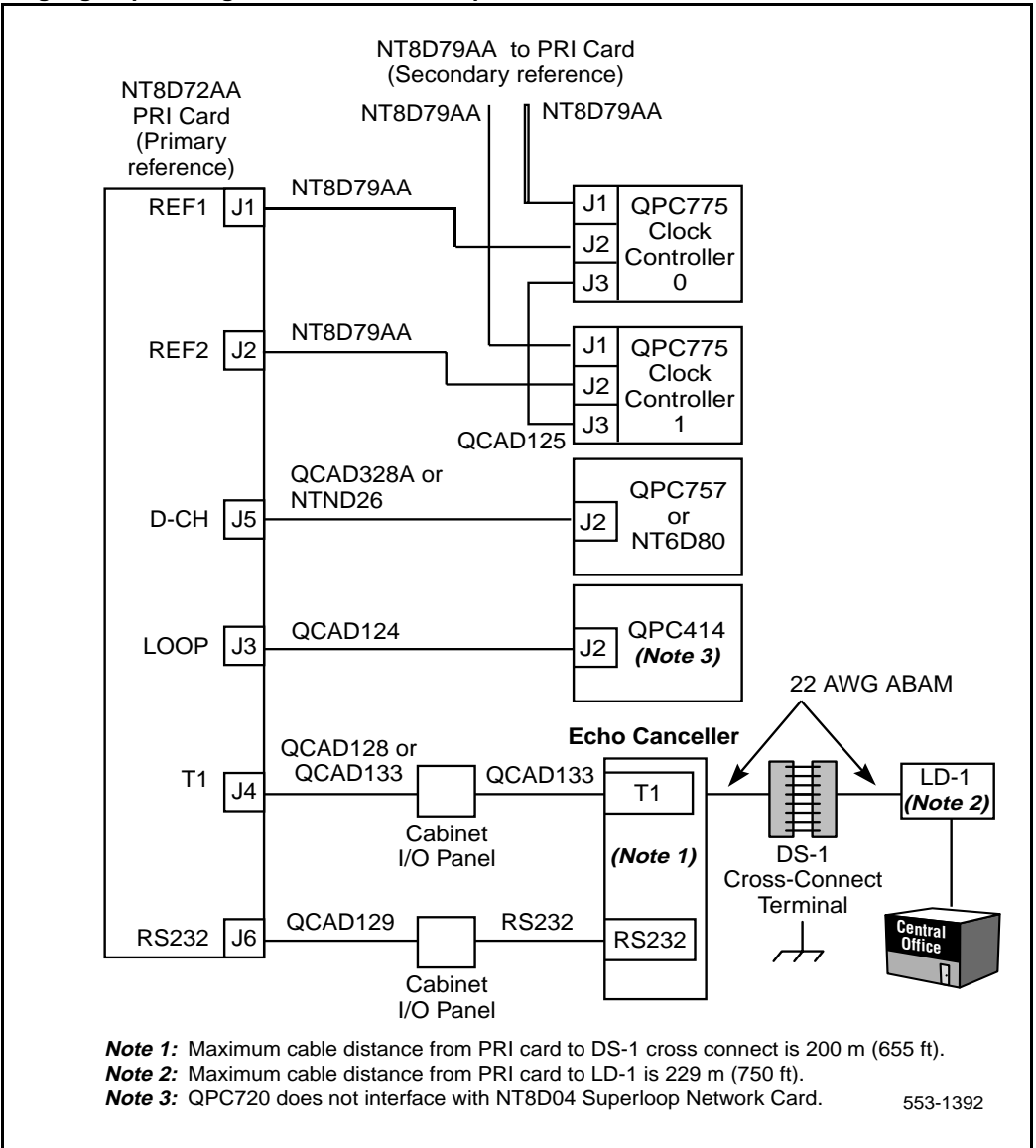
Figure 54 Single group cabling for the NT8D72 on Options 51C and 61C, with echo canceller
