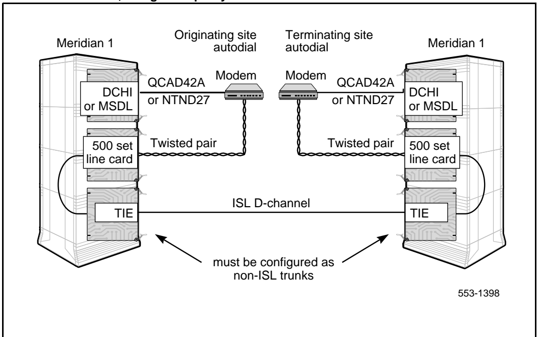
Figure 84 ISL dedicated mode, using dial-up Hayes Smartmodem 2400
