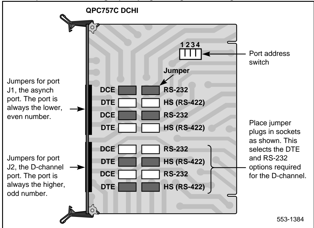
Figure 48 QPC757 option and PRI/ISL high speed programming switch settings
