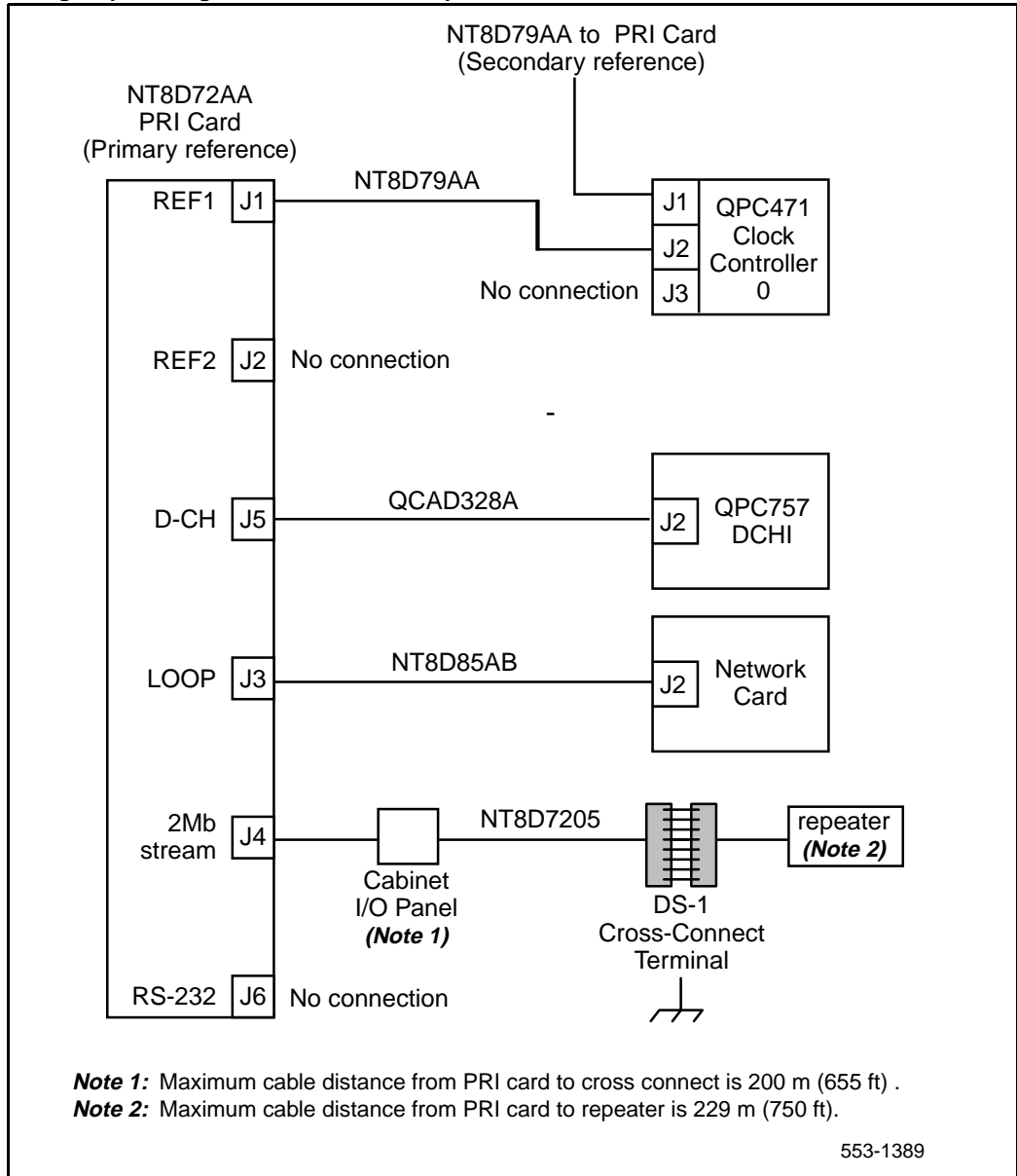
Figure 51 Half-group cabling for the NT8D72 on Options 51C and 61C, without an echo canceller
