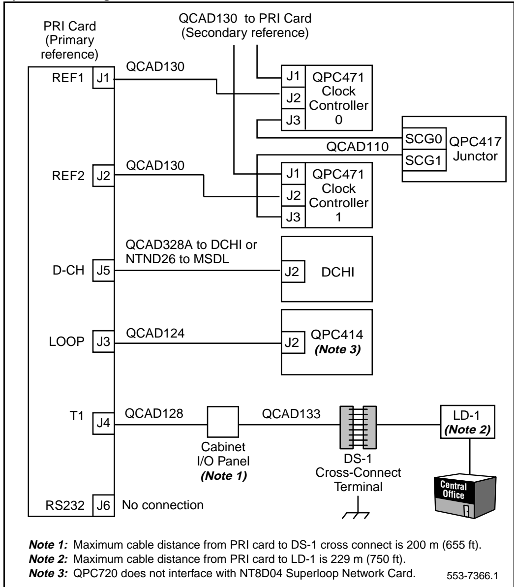
Figure 61 Option 81C cabling for the QPC720 without echo canceller
