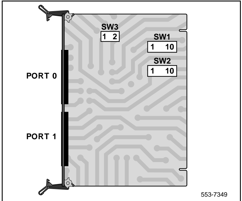
Figure 45 NT6D11 DIP switches
