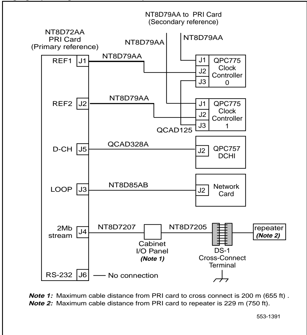
Figure 53 Single-group cabling for the NT8D72 on Options 51C and 61C, without echo canceller
