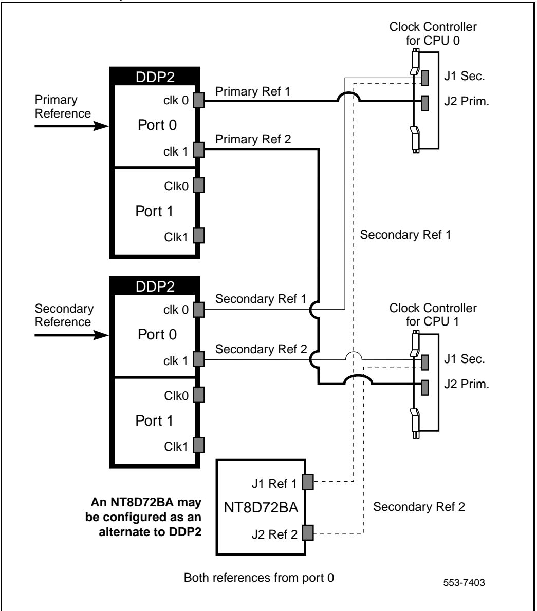
Figure 33 Clock Controller – Option 2
