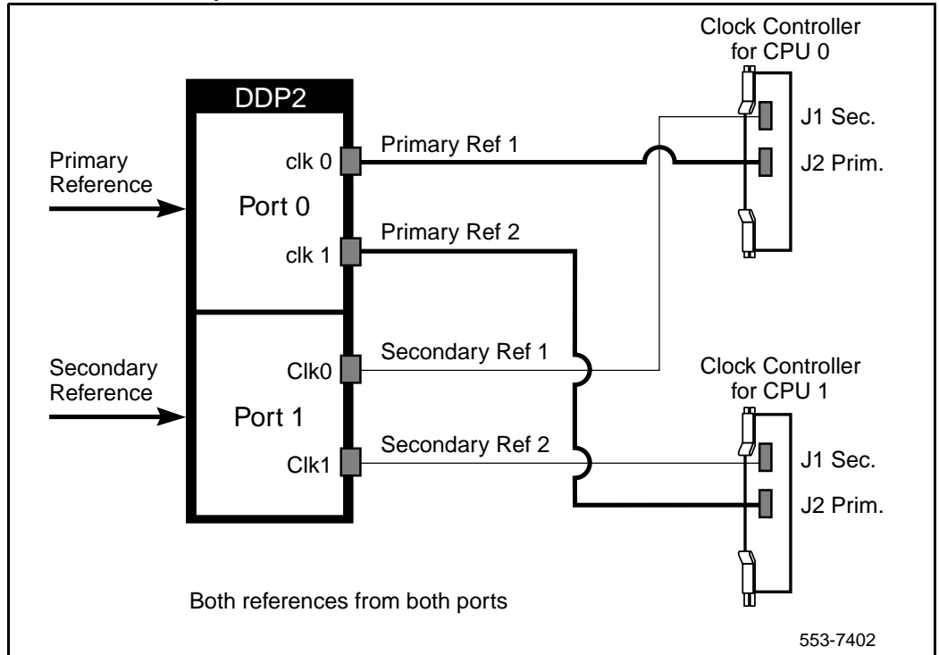
Figure 35 Clock Controller – Option 4
