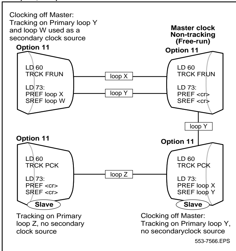
Figure 76 Example 6, Complex Isolated Private Network
