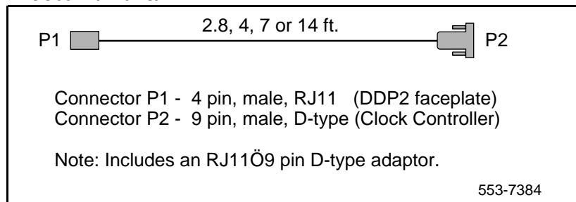
Figure 26 NTCG03AA/AB/AC/AD
