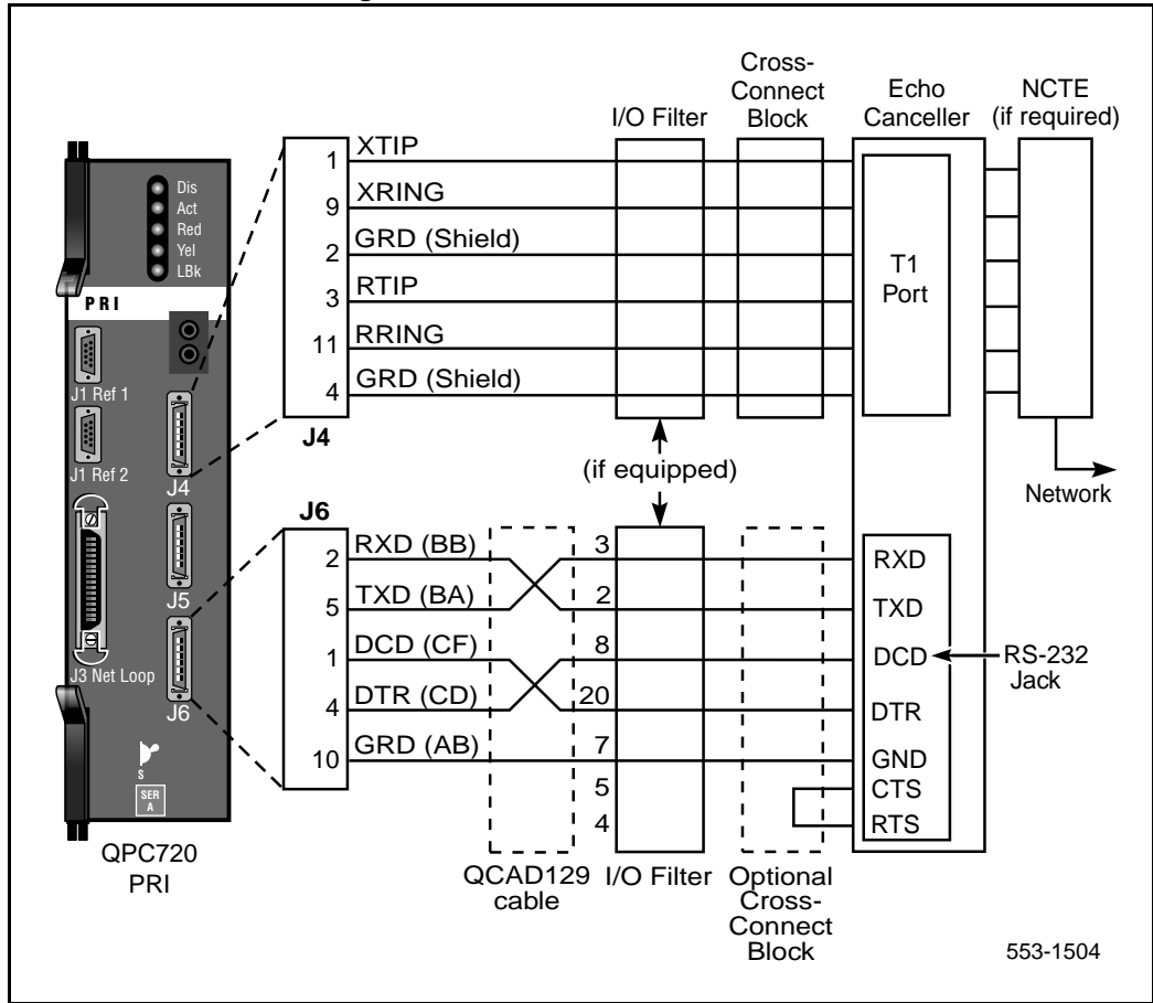
Figure 86 PRI to echo canceller cabling
