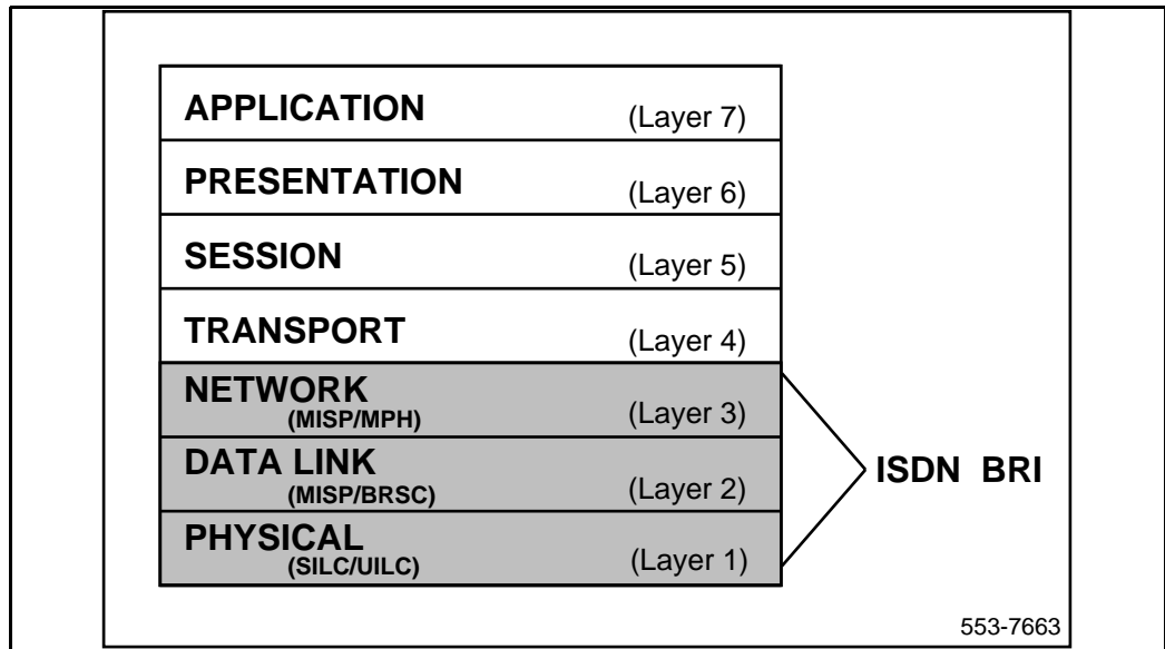
Figure 1 OSI model
