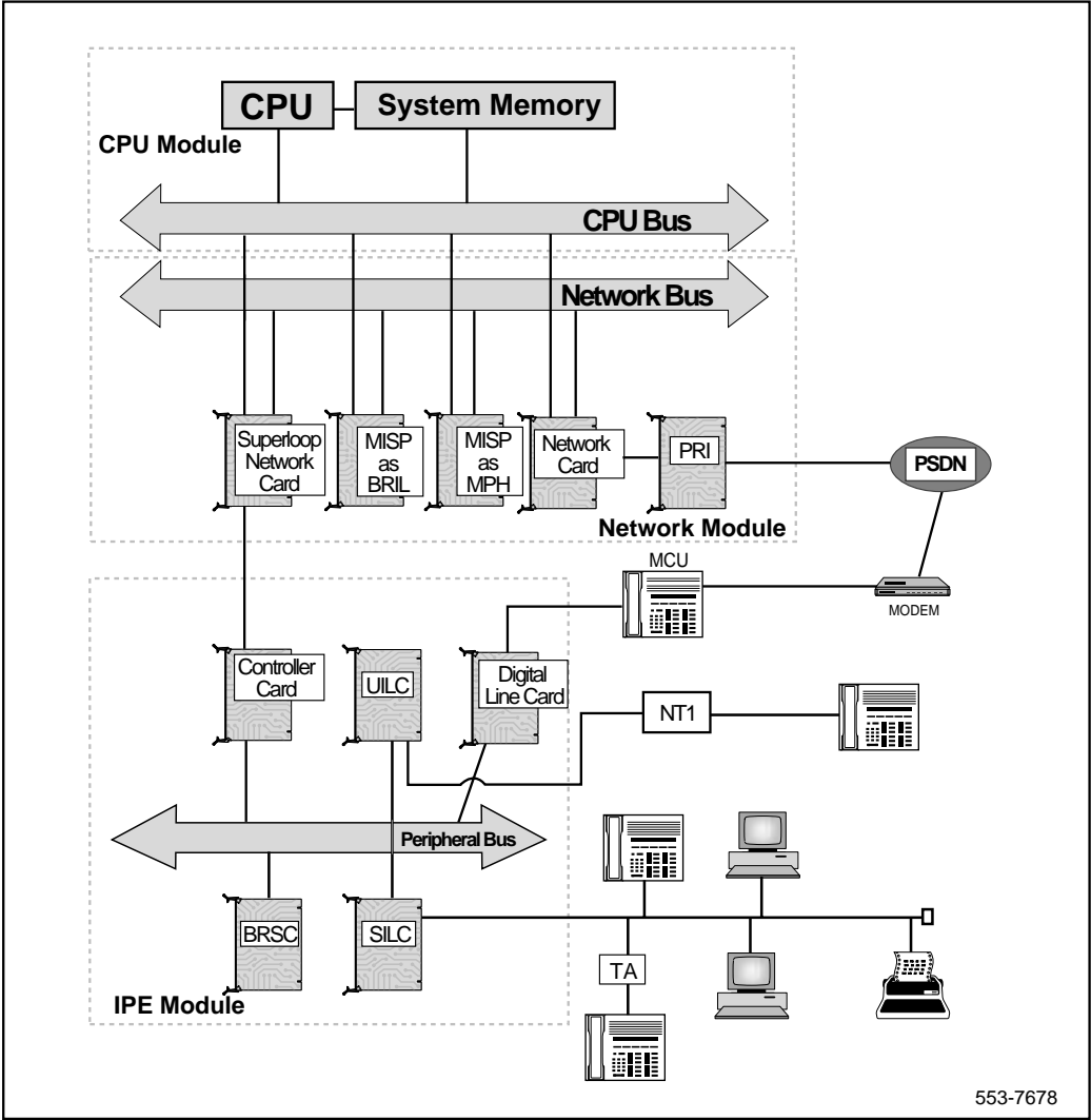
Figure 16 A basis ISDN BRI MPH packet data architecture, with a BRSC and an MCU
