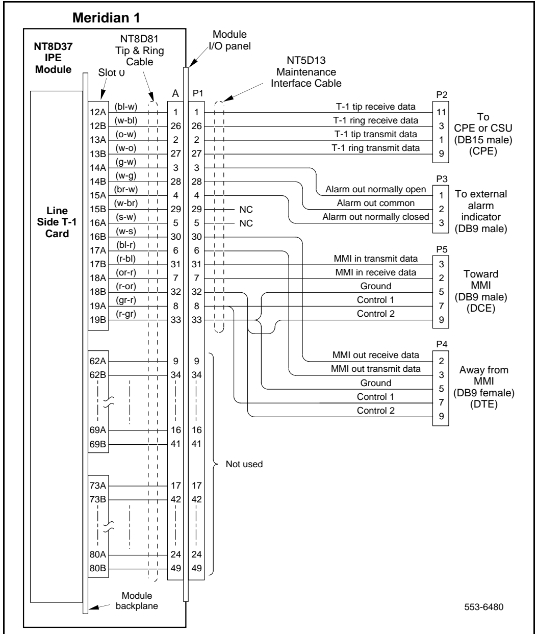
Figure 18 Line-side T1 card – connection using the NT5D13AA Line-side T1 Cable
