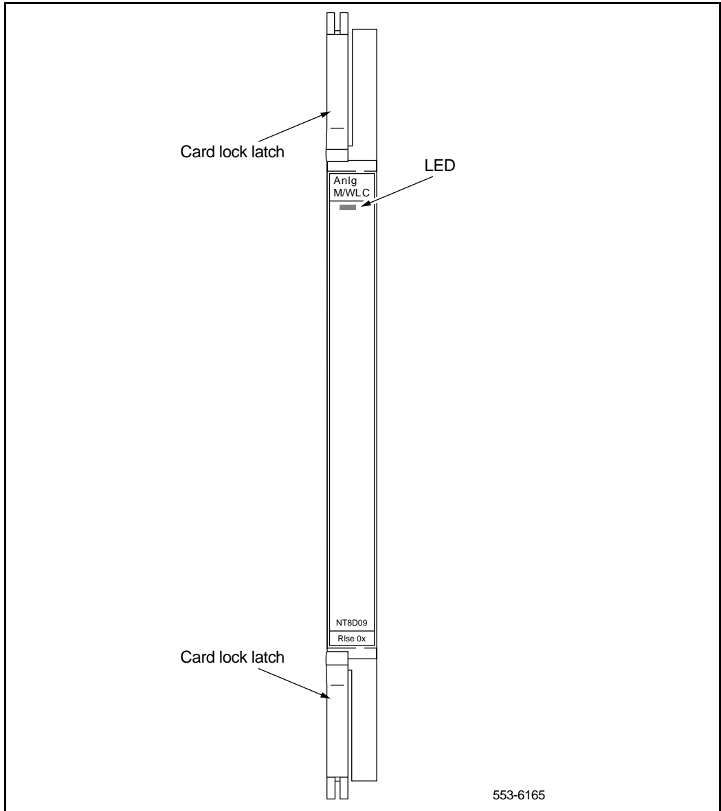
Figure 53 Analog message waiting line card – faceplate
