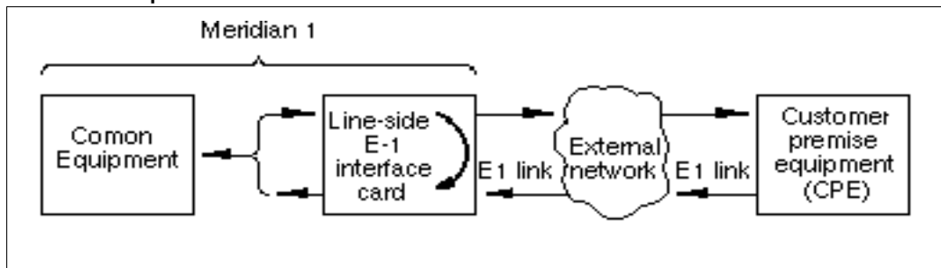
Figure 44 MMI Local loopback test
