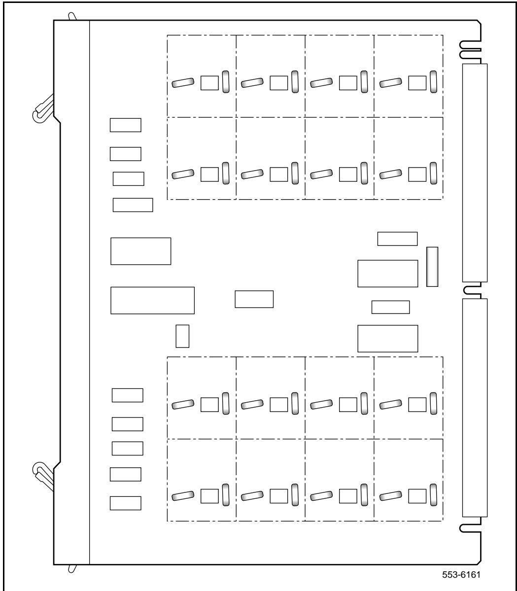
Figure 52 Digital line card – jumper block and switch locations.
