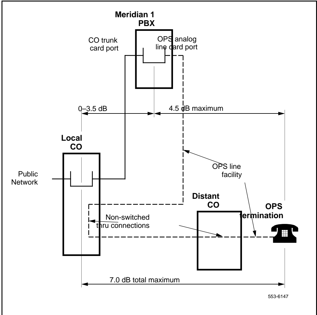
Figure 14 Traditional OPS application configuration
