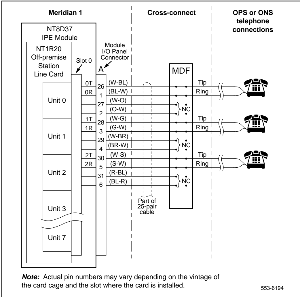
Figure 12 OPS analog line card – typical cross connection example
