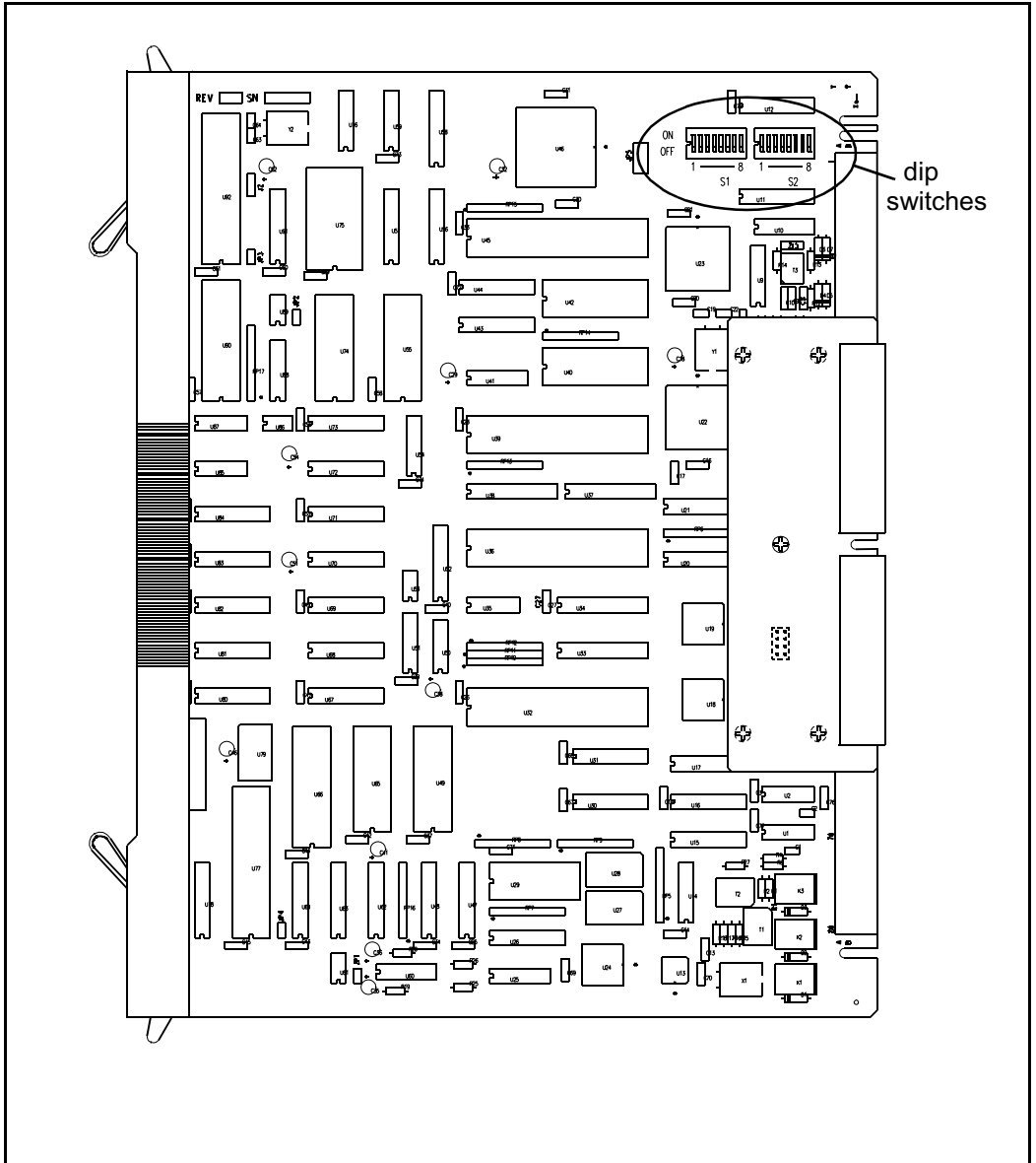
Figure 29 Line-side E1 card – E1 protocol dip switch locations
