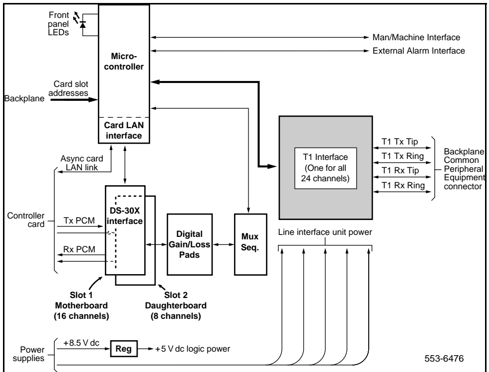
Figure 16 Line-side T1 card – block diagram
