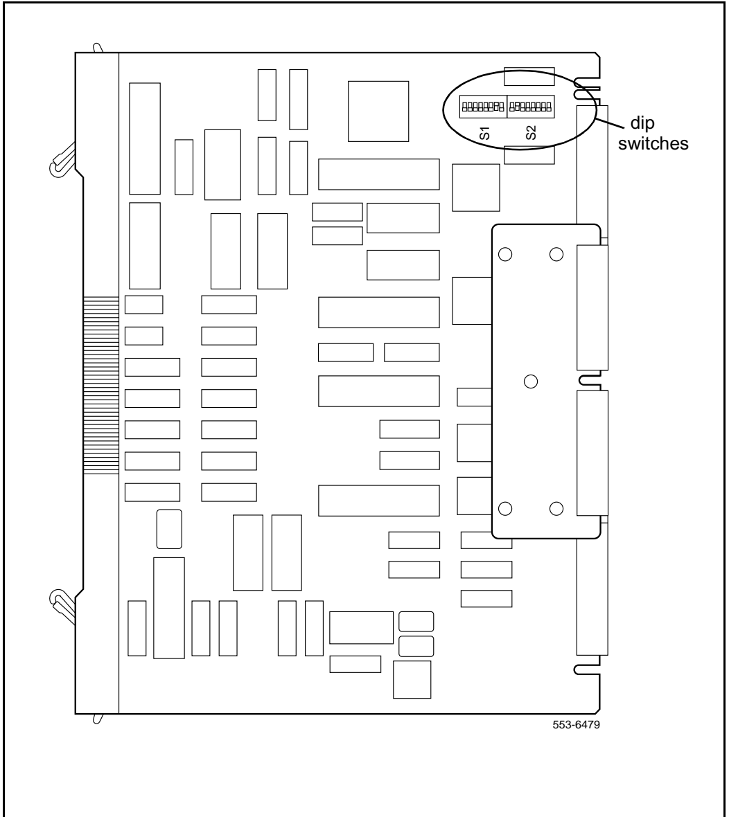
Figure 17 Line-side T1 card – T1 protocol dip switch locations
