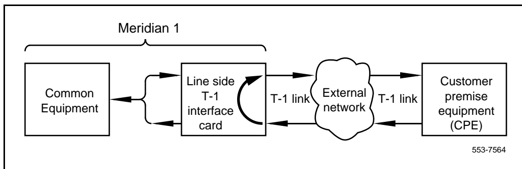
Figure 22 MMI Network loopback test
