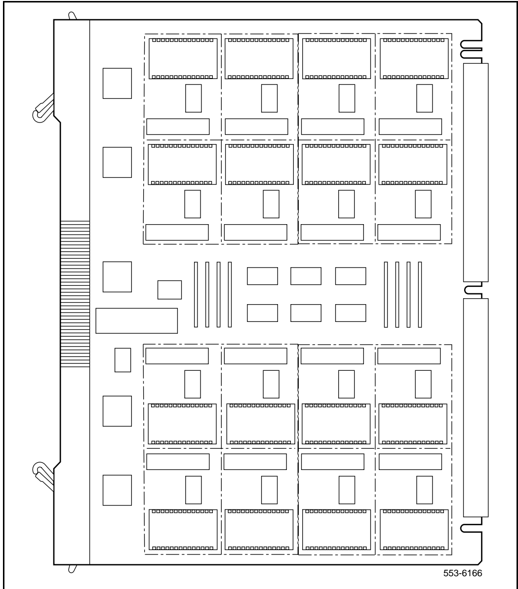
Figure 56 Analog message waiting line card – jumper block and switch locations
