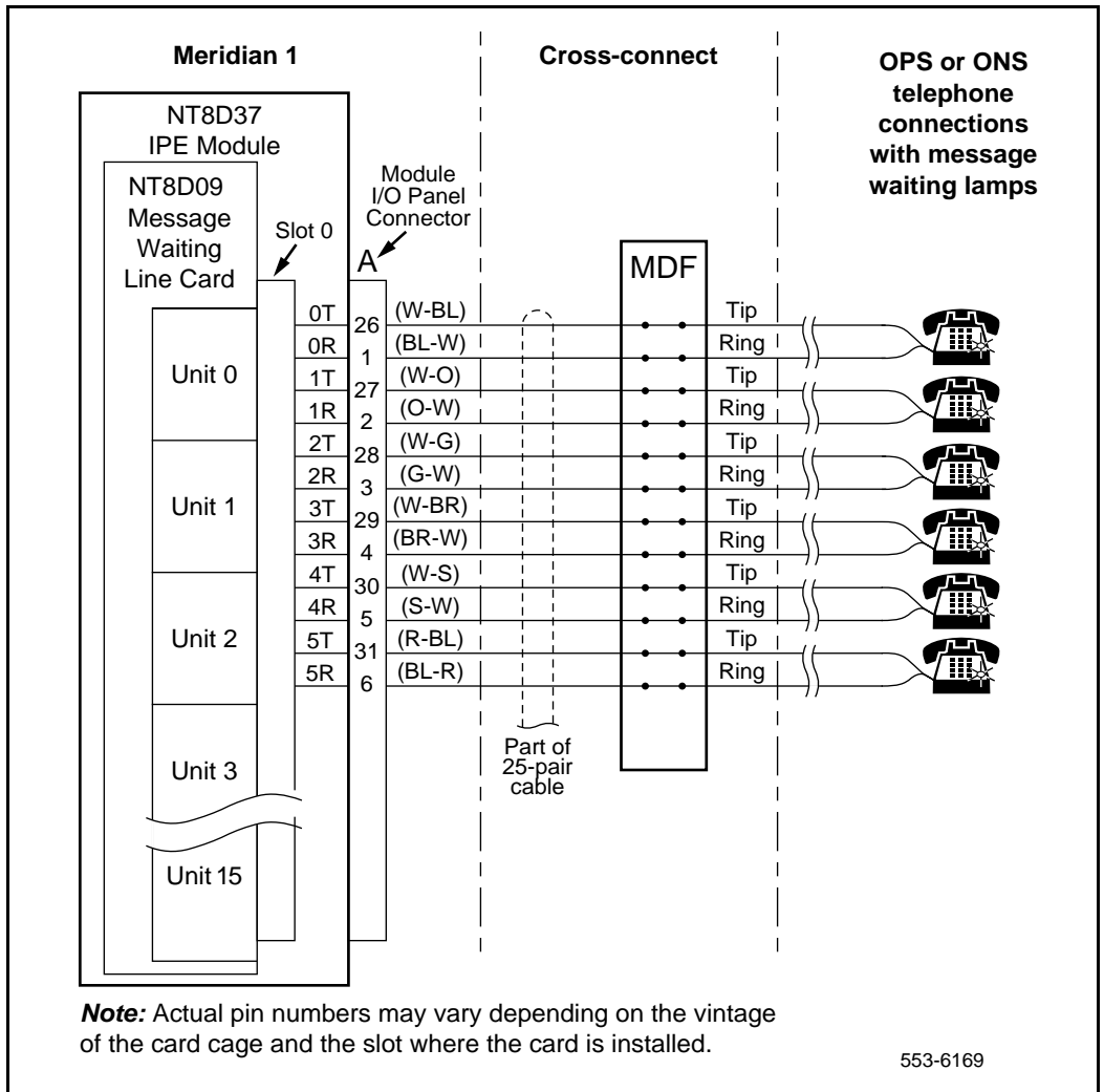
Figure 55 Analog message waiting line card – typical cross connection example
