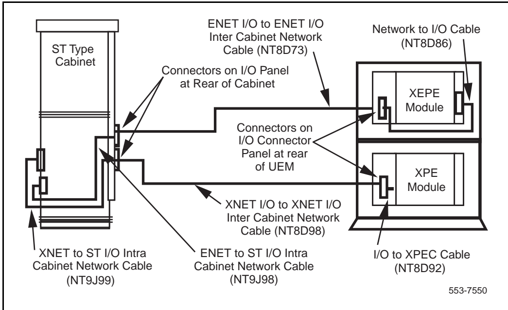
Figure 21 ST to module intercabinet cabling
