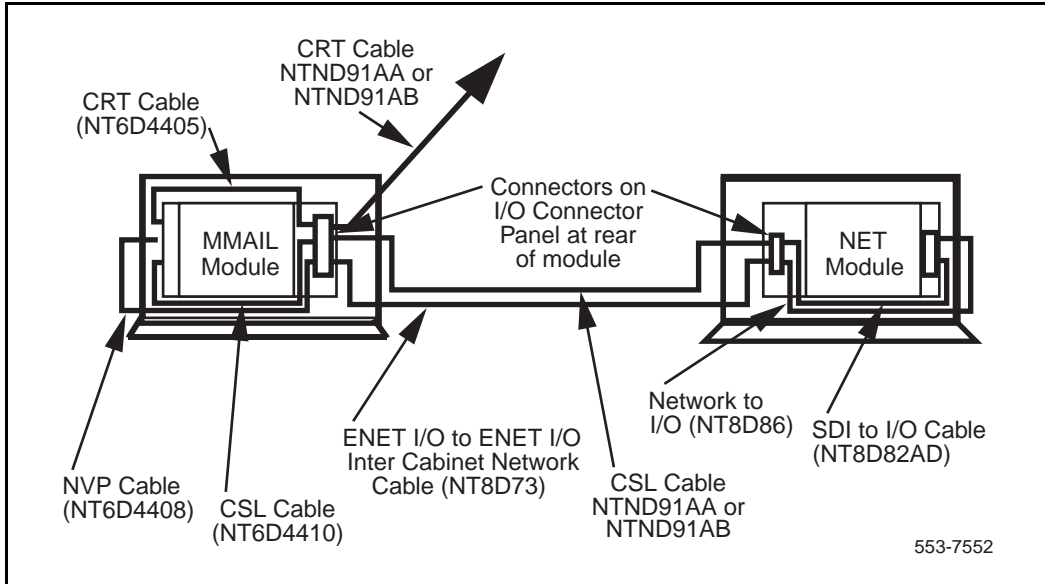
Figure 23 Meridian Mail module cabling
