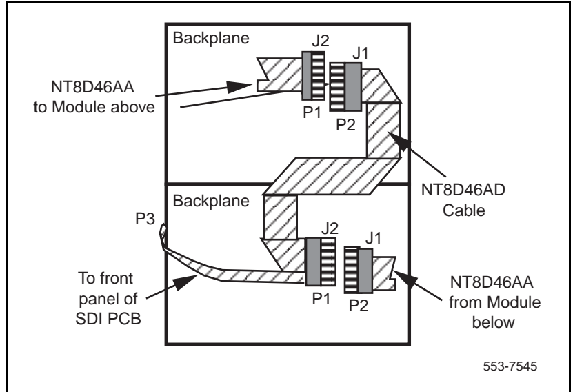
Figure 16 System monitor to SDI cabling method
