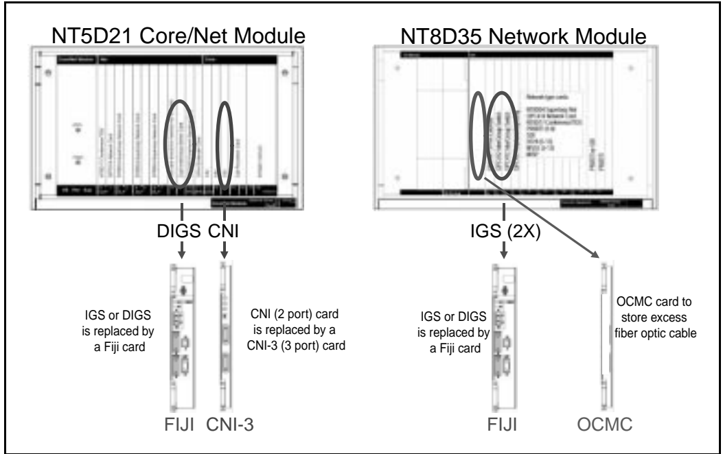
Figure 27 Option 81C Fiber Network upgrade
