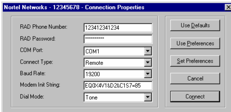
Figure 3 Connection Properties screen
