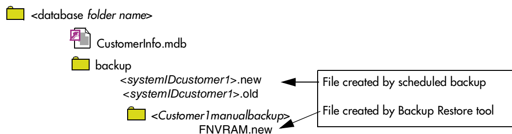
Figure 18 Customer database backup folders
