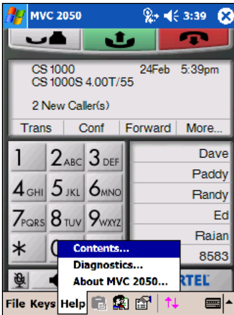
Figure 14: Help menu
