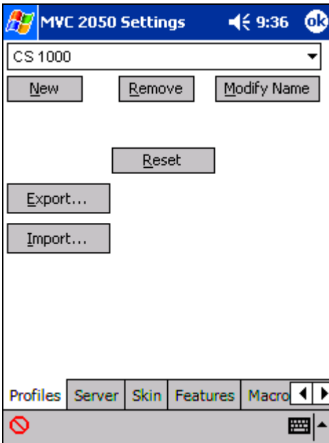
Figure 27: Profiles screen
