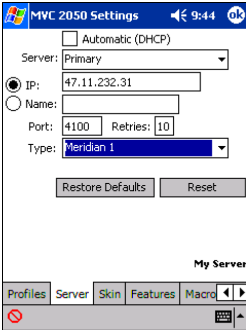
Figure 29: Server screen
