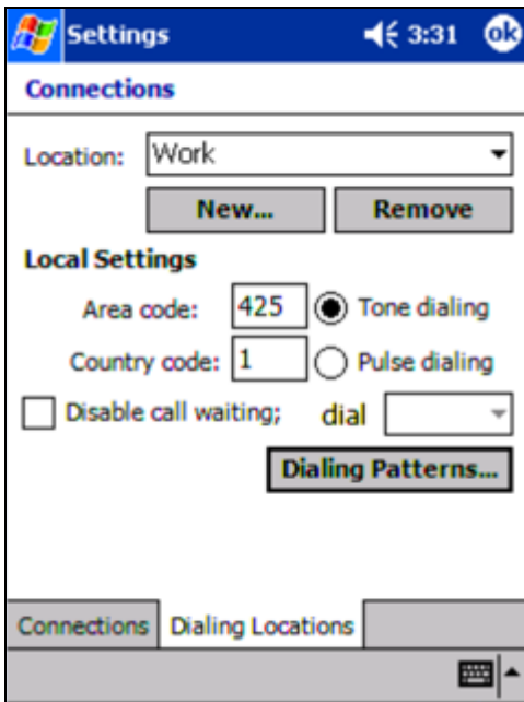
Figure 21: Dialing locations
