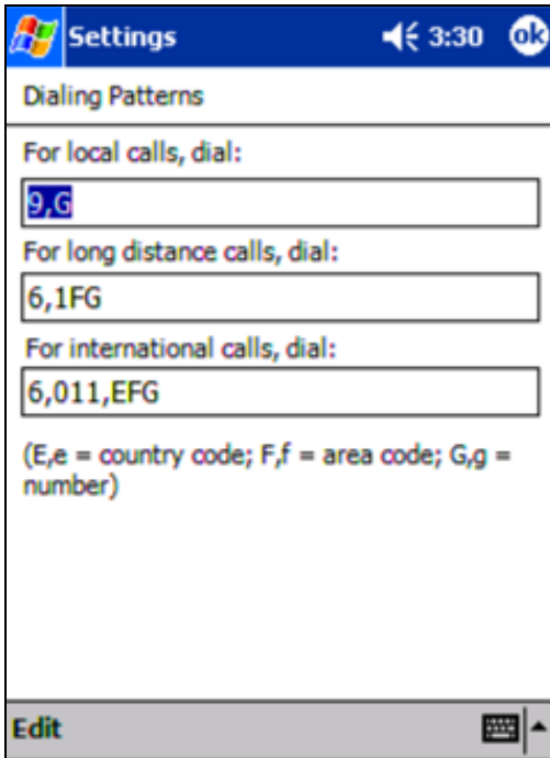
Figure 22: Dialing patterns
