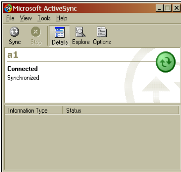
Figure 4: ActiveSync connected
