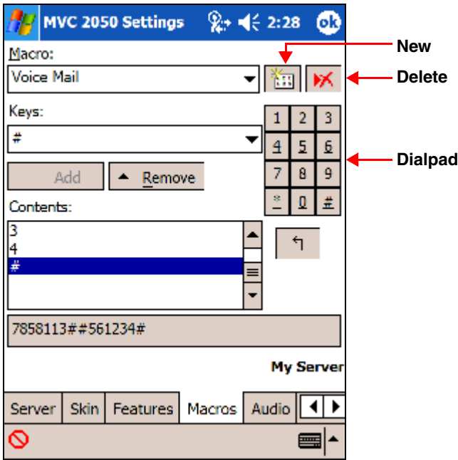
Figure 32: Macro screen
